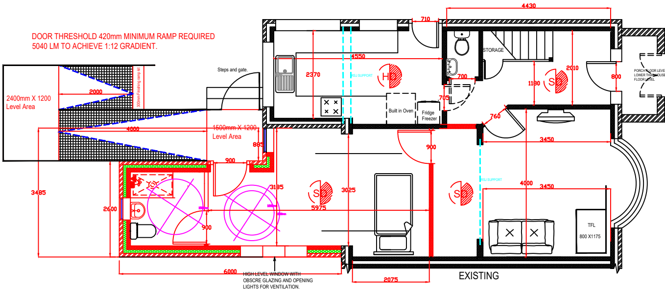
PROPOSED GROUND FLOOR LAYOUT.
