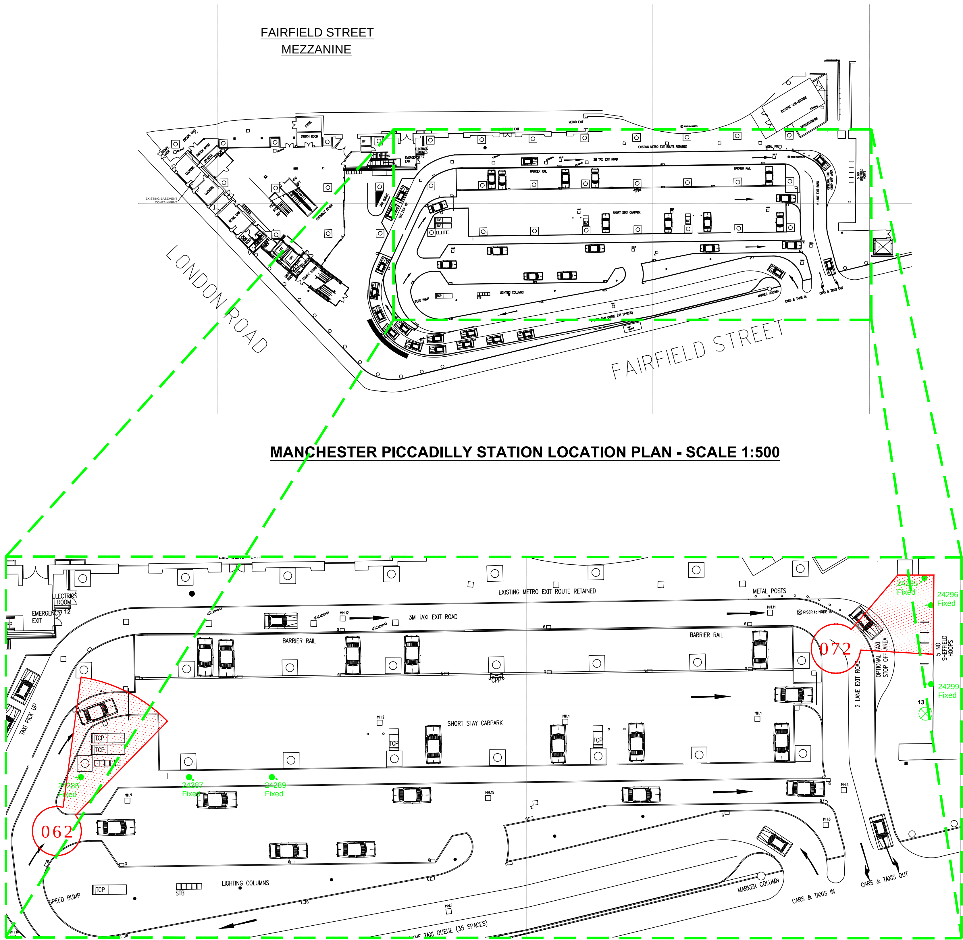
MANCHESTER PICCADILLY STATION PLAN FAIRFIELD STREET - SCALE 1:250
