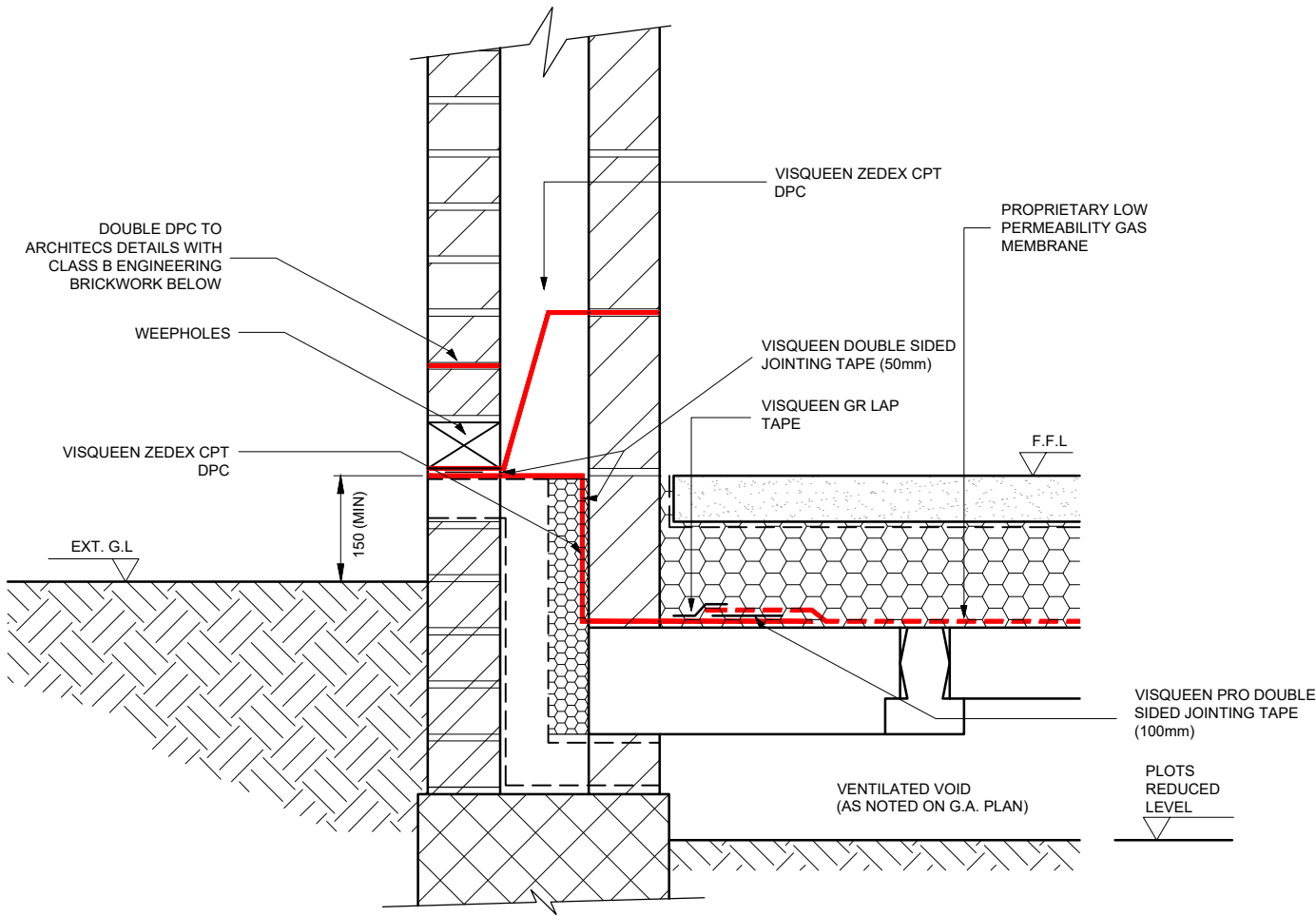
Detail Scale- 1:10
