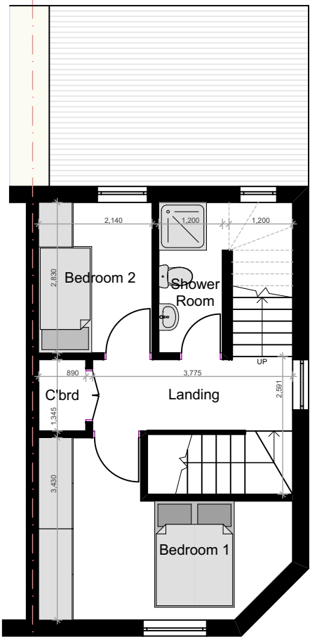
PROPOSED GA FIRST FLOOR PLAN
