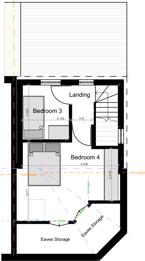
PROPOSED GA SECOND FLOOR PLAN
