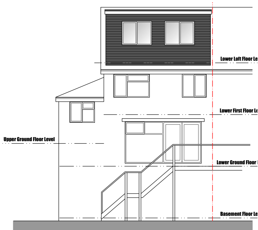
North West Facing Rear Elevation
