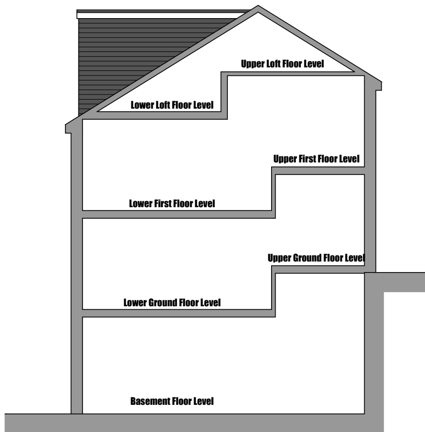
South West Facing Side Elevational Section
