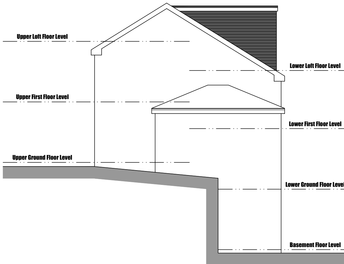
North East Facing Side Elevation
