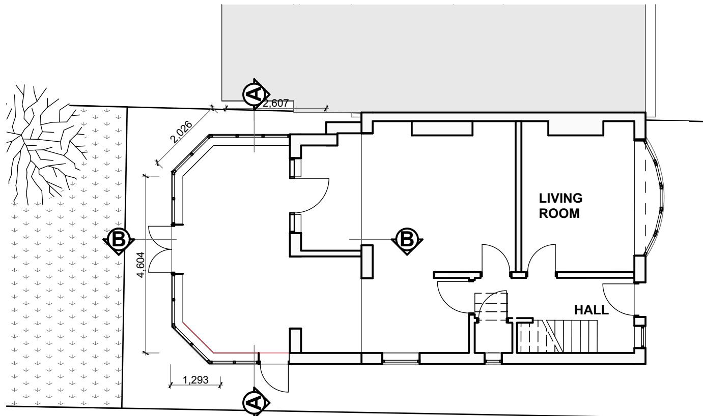
EXISTING GROUND FLOOR 1:100
