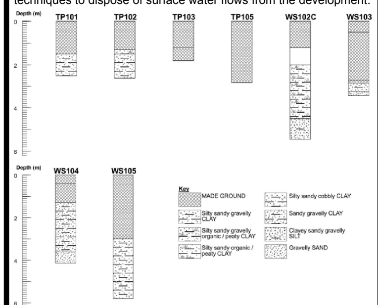
Plate 4-1: Summary of ground conditions.
