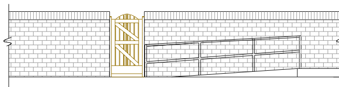
PROPOSED ELEVATION C
