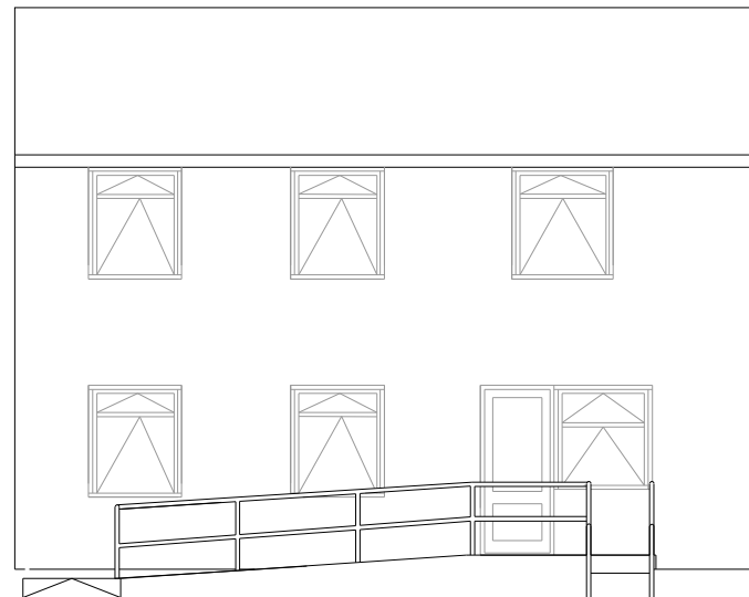
PROPOSED ELEVATION A
