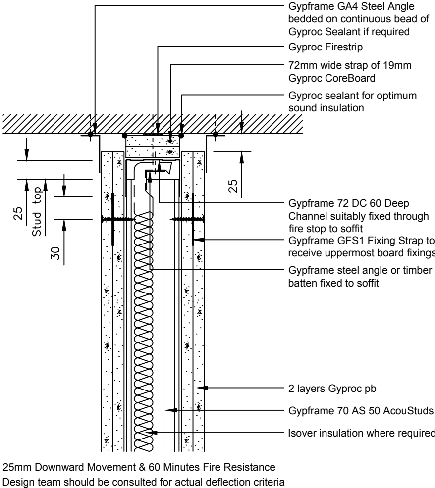
Typical Deflection Head Detail 1:5
