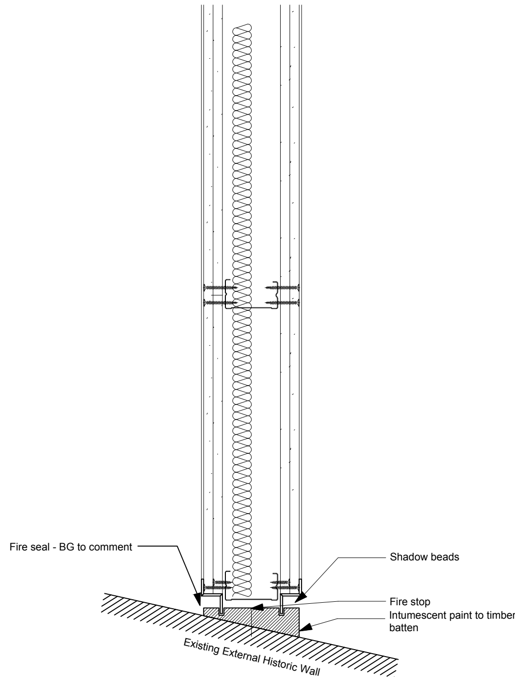
Typical Proposed to Existing Wall Element Abutment Detail 1:5
