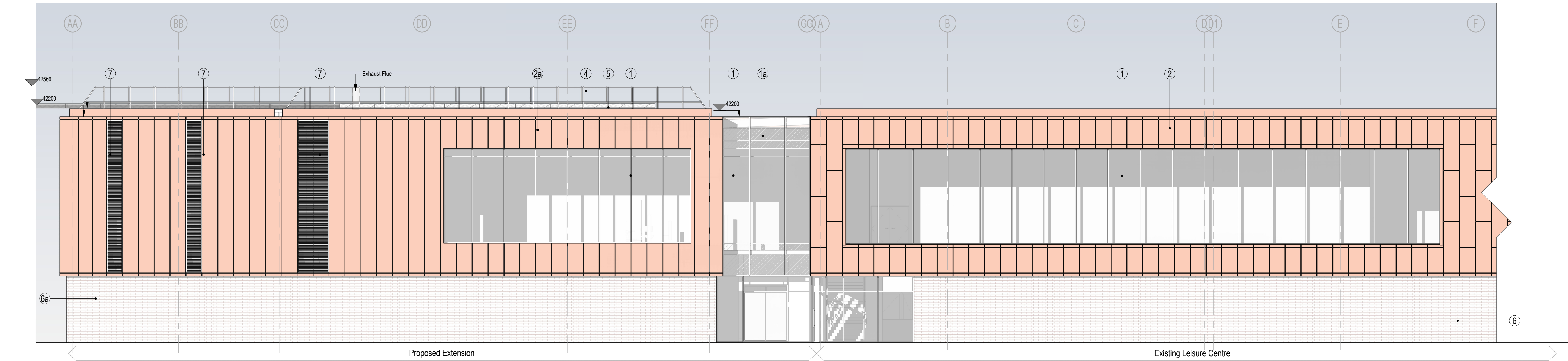
2 Elevation 02 - East
