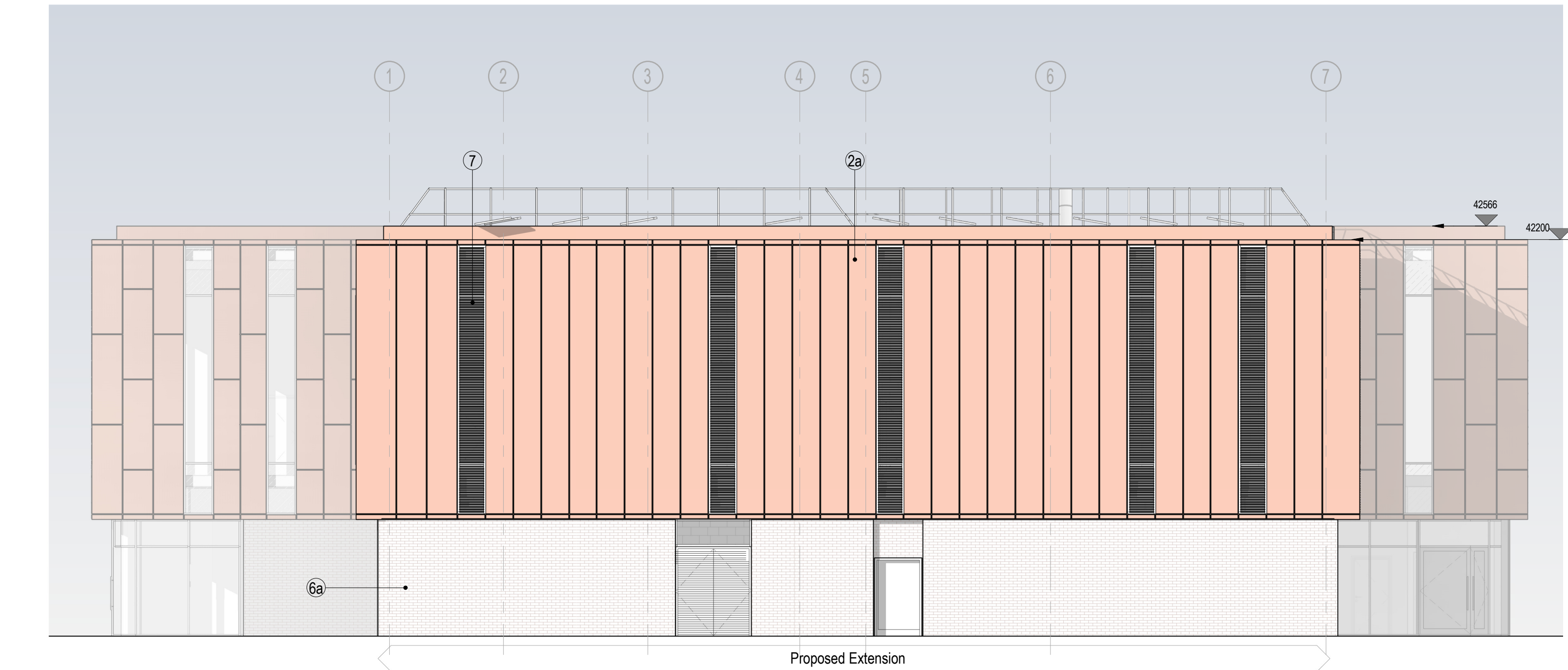
3 Elevation 03 - South
