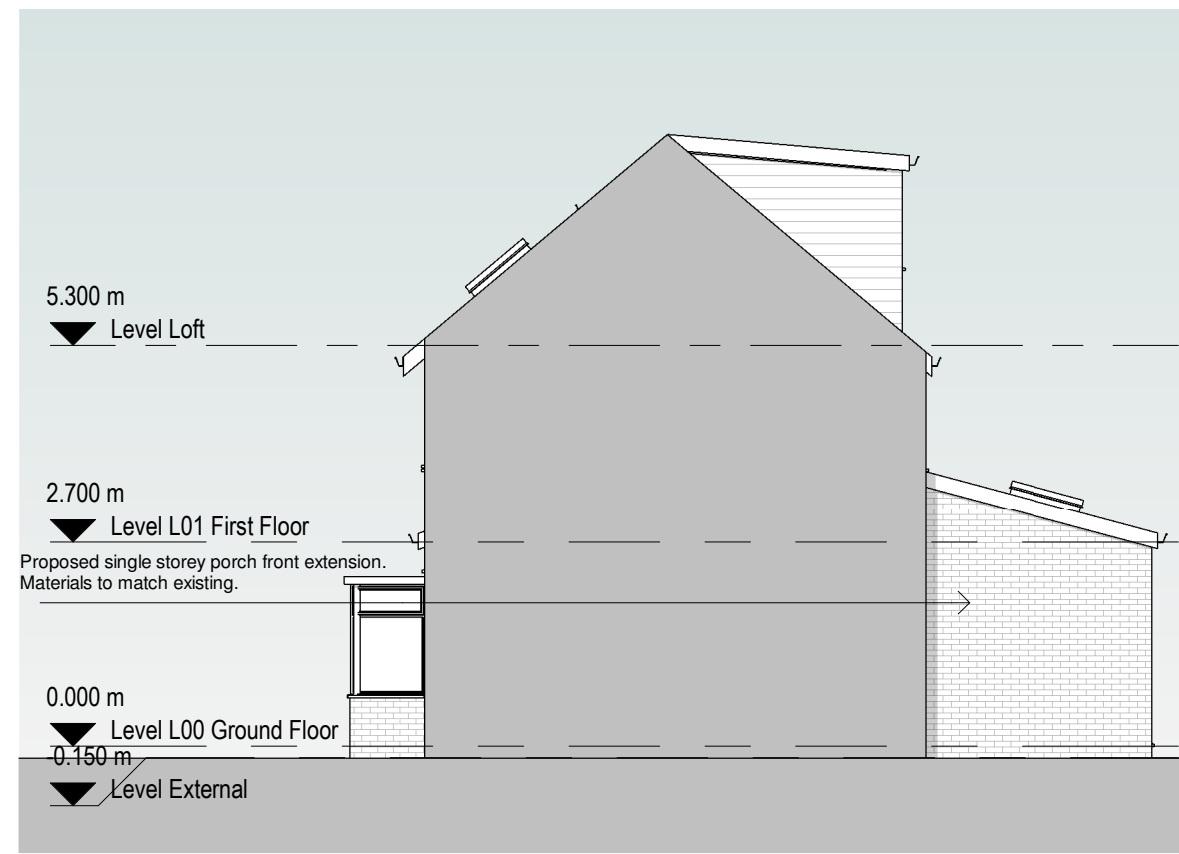
4 Proposed East Elevation 1 : 100
