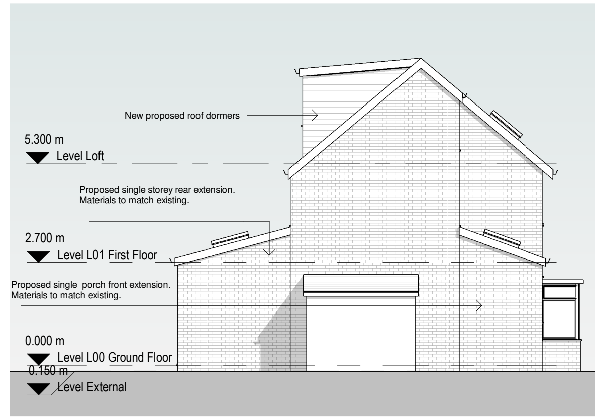
2 Proposed West Elevation 1 : 100
