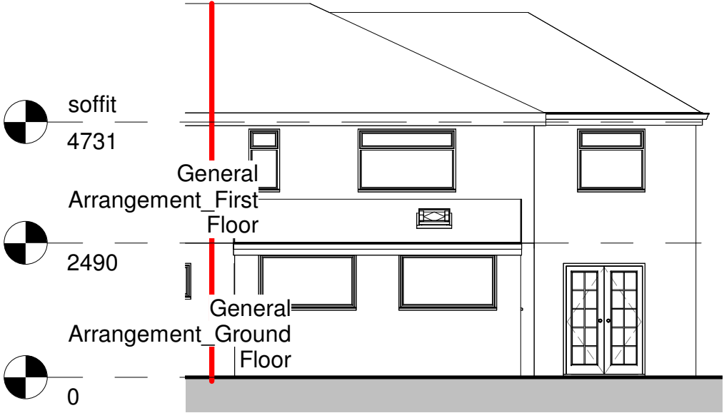
Proposed Elevation East 1 : 100
