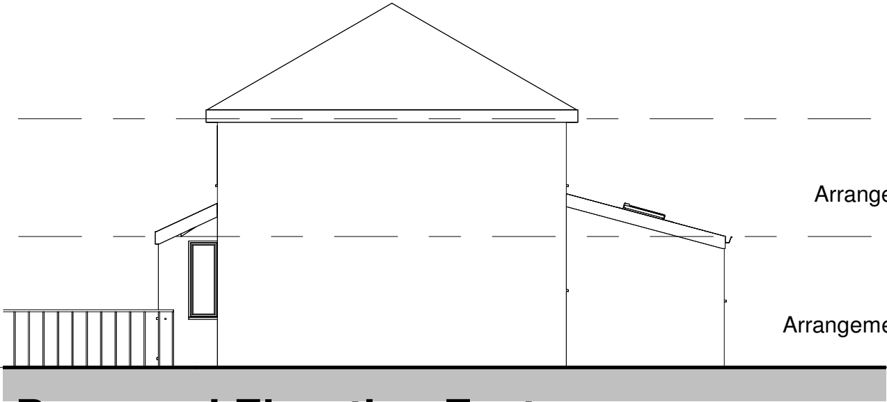
Proposed Elevation East 1 : 100
