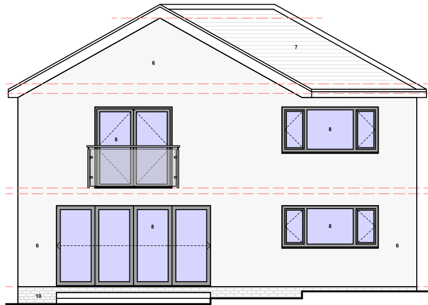
PROPOSED GA REAR ELEVATION
