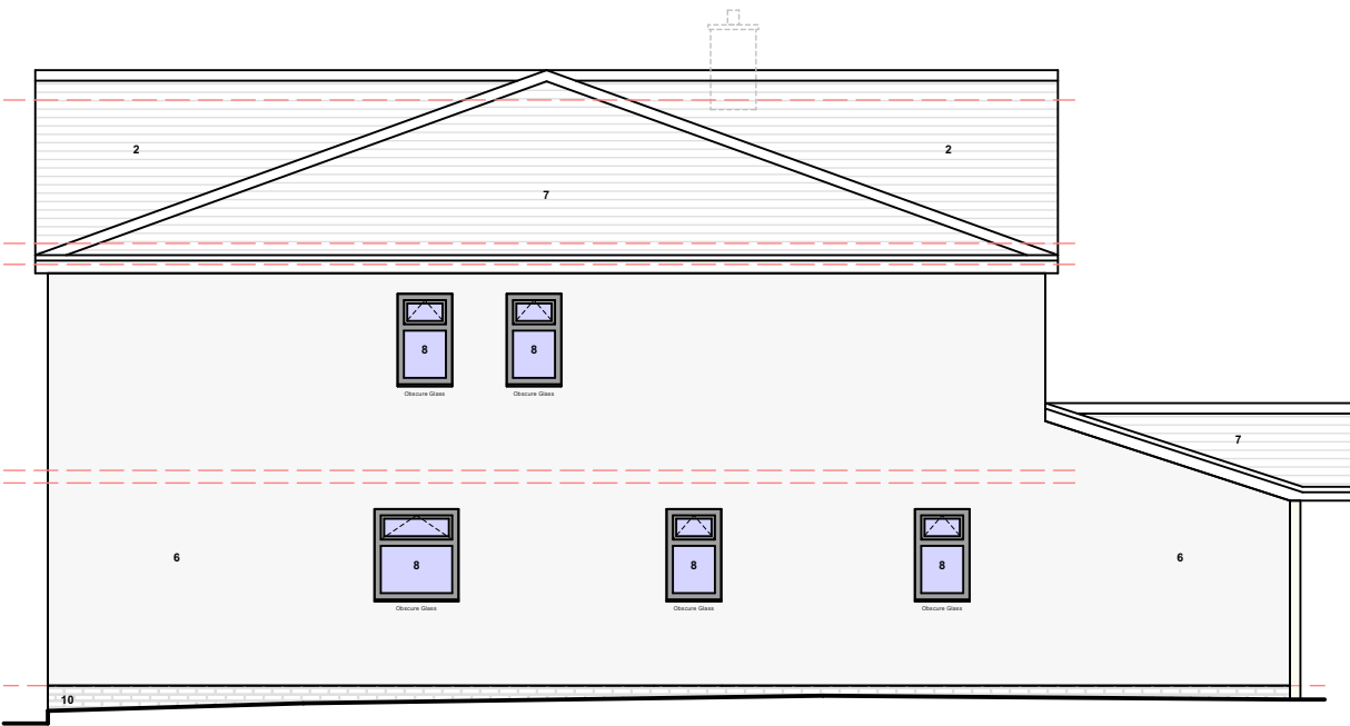
PROPOSED GA SIDE ELEVATION 1
