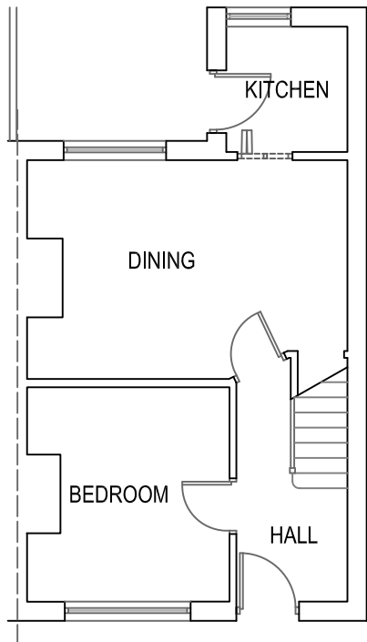
EXISTING GF PLAN 1:100 @ A3
