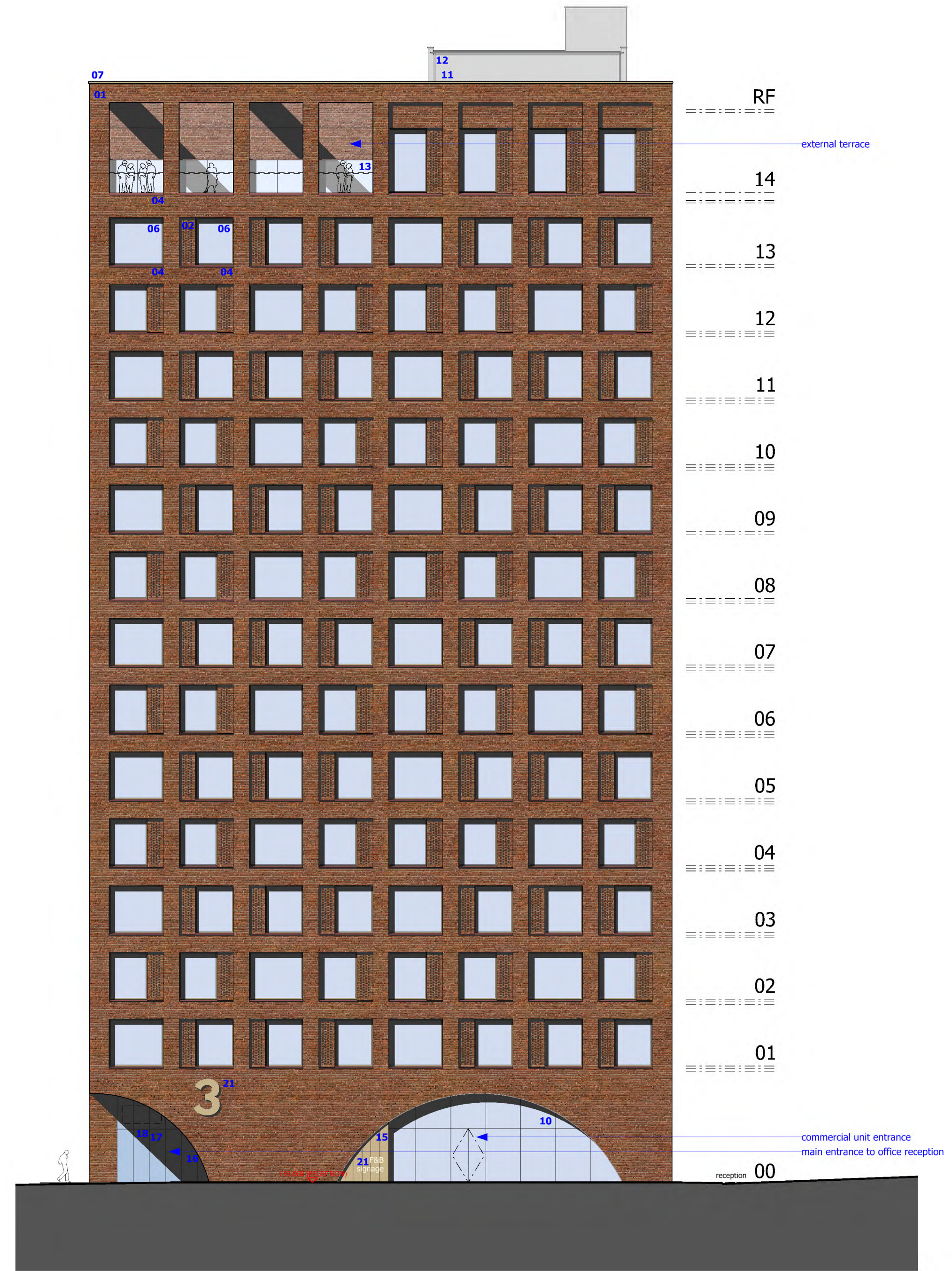
PROPOSED ELEVATION - WEST (1:200)
