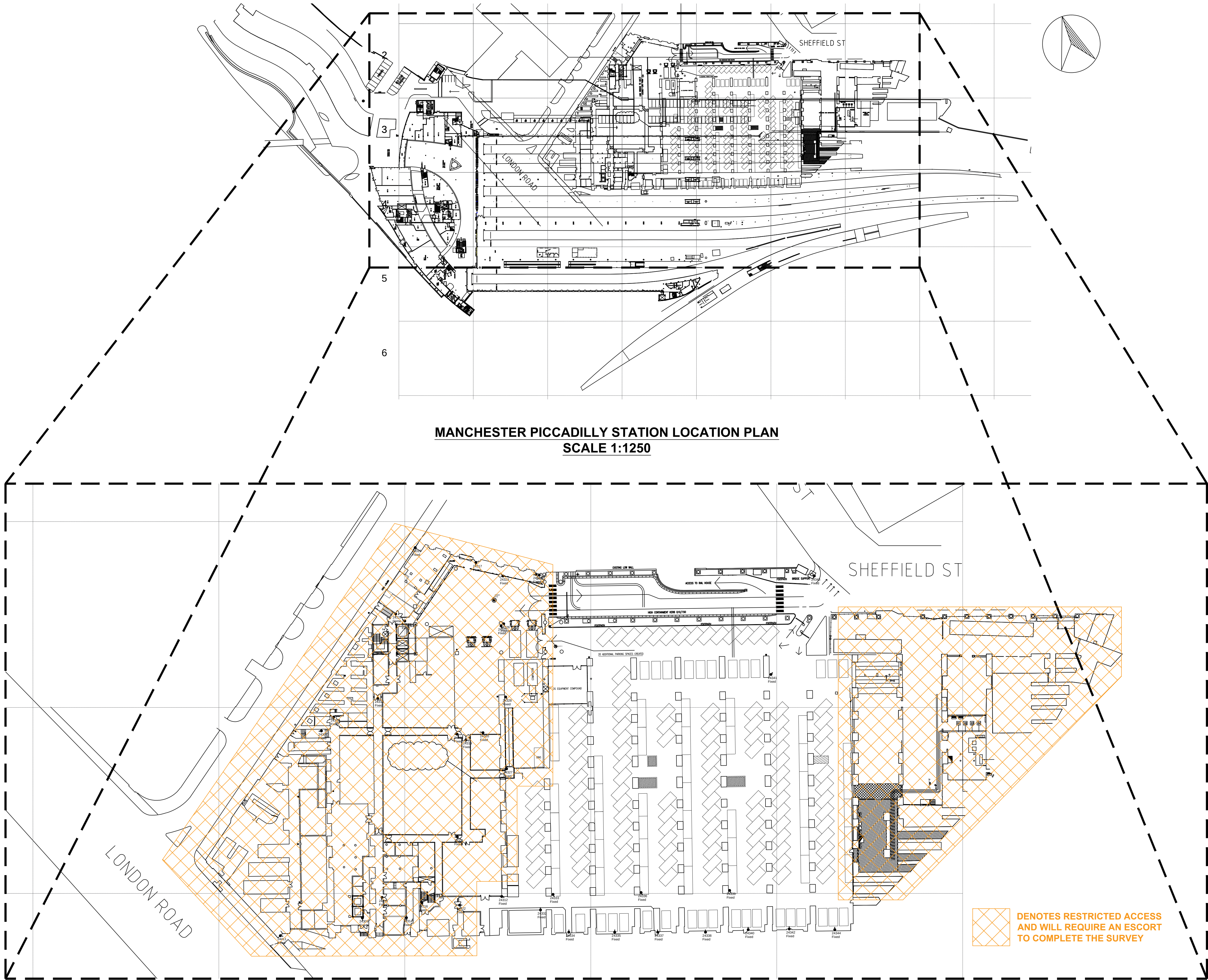
MANCHESTER PICCADILLY STATION PLAN UNDERCROFT - SCALE 1:500
