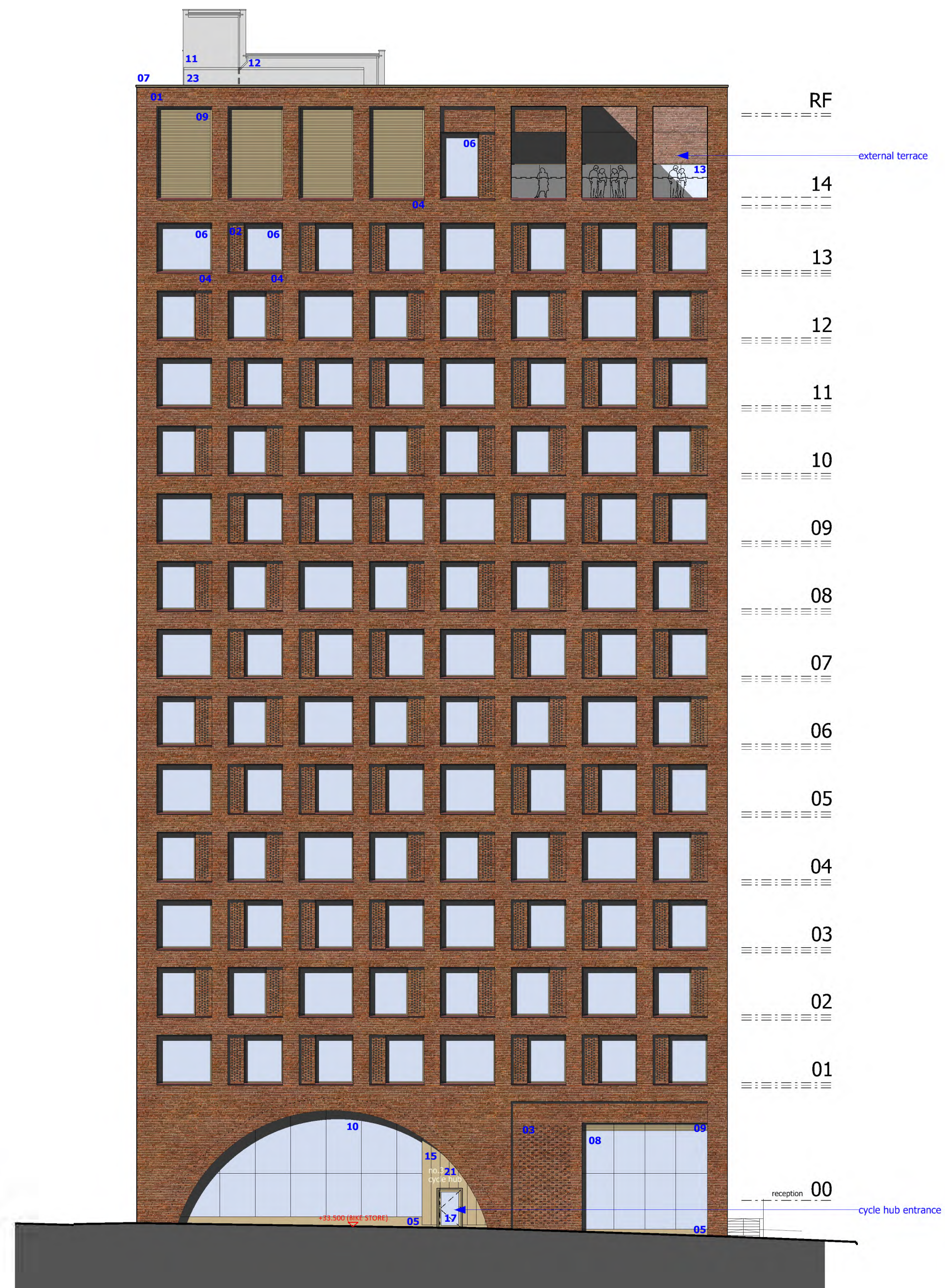
PROPOSED ELEVATION - EAST (1:200)
