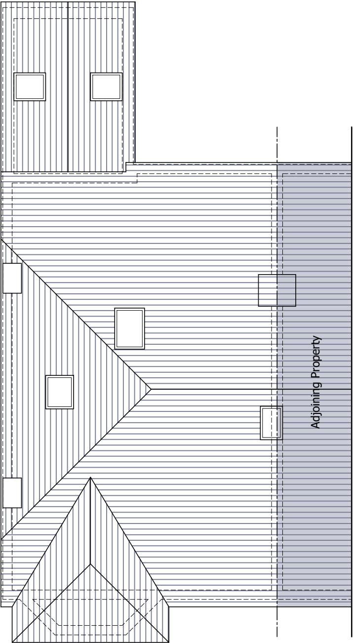
ROOF PLAN
