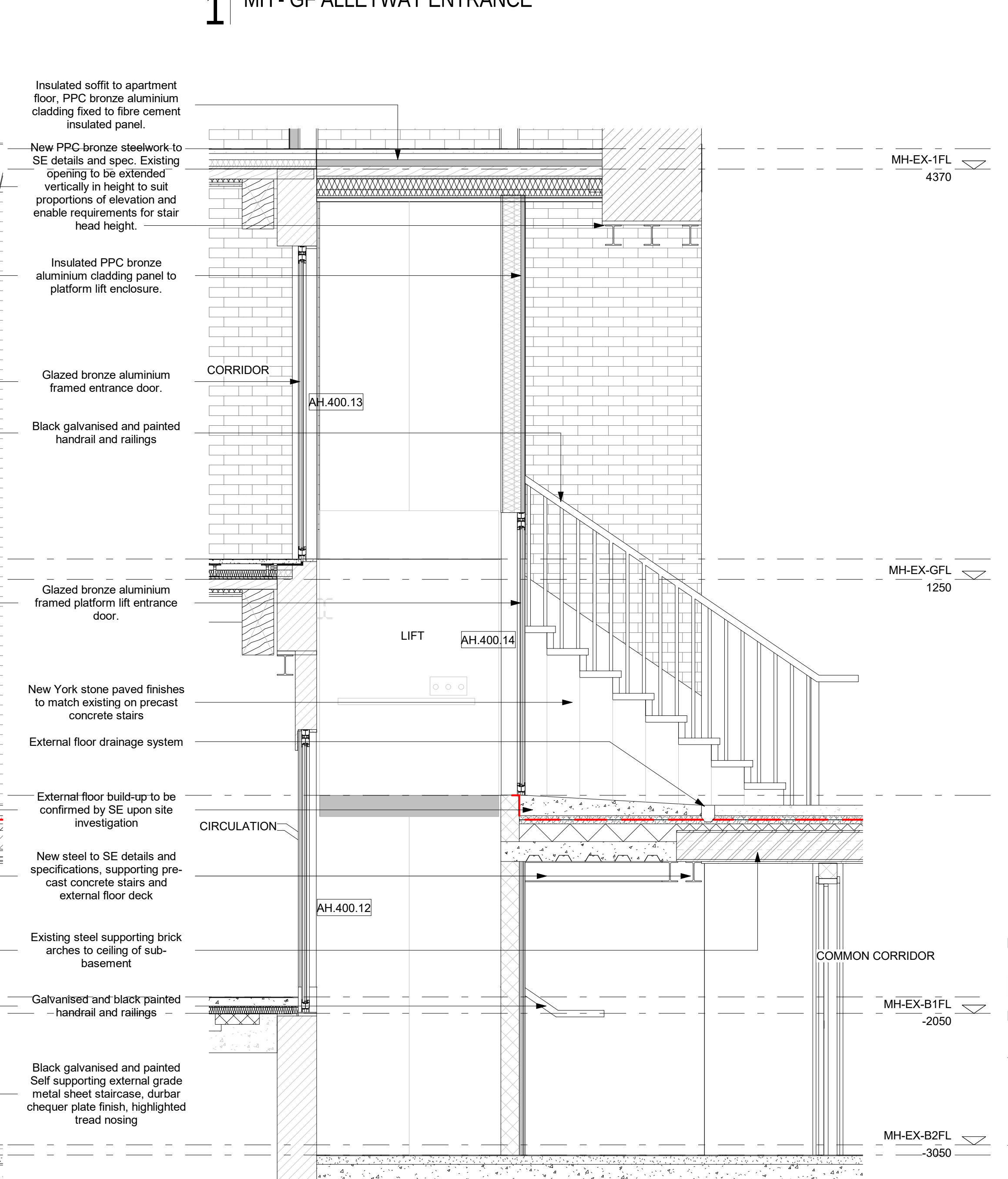
B | MH - ALLEYWAY ENTRANCE PLATFORM LIFT SECTION
