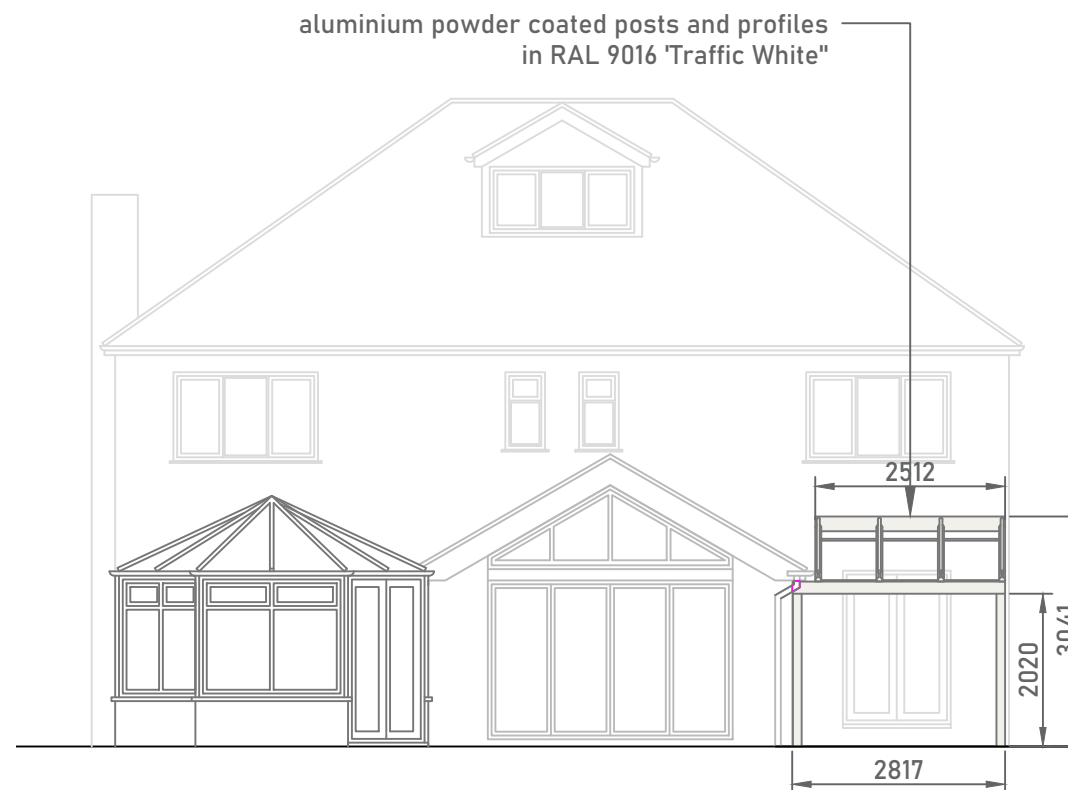
REAR ELEVATION
