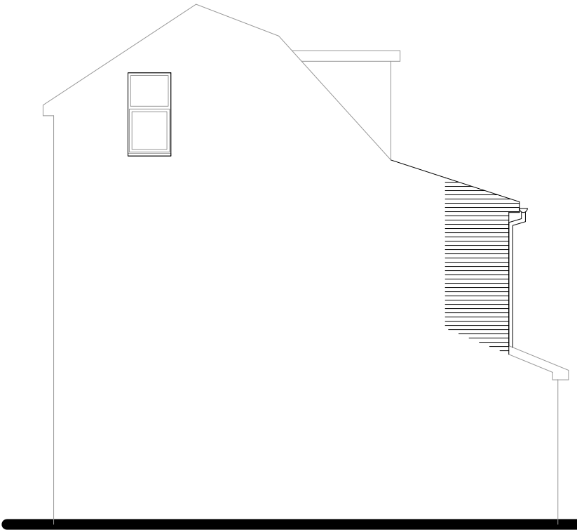
Side Elevation
