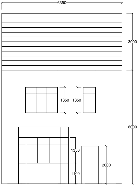
Front Elevation as Existing
