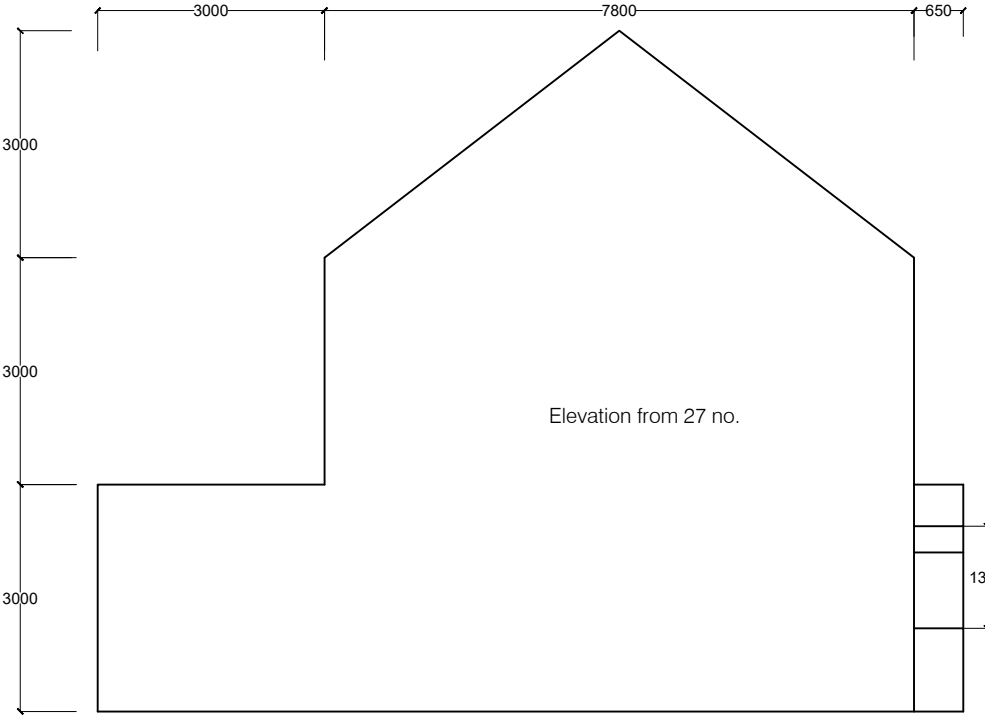
North Elevation as Existing
