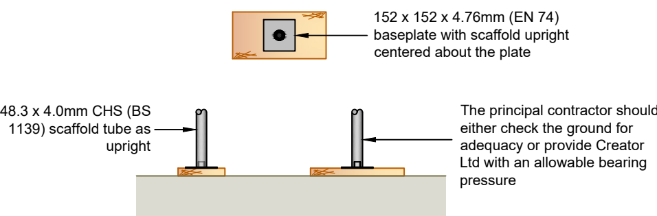
FOUNDATION DETAIL 225 x 38 x 450mm (BS EN 2482) Scaffold Board Solepad Scale - 1:25
