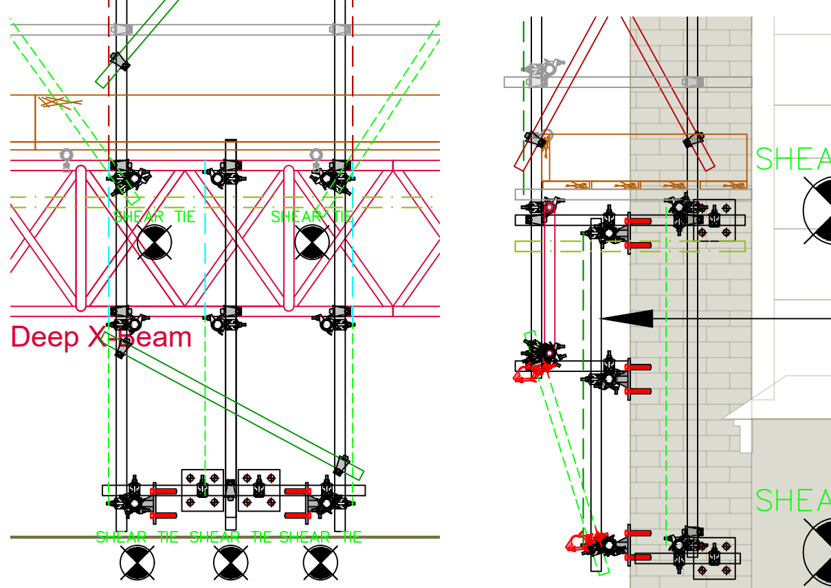
GALLOWS BRACKET DETAIL scale 1:25
