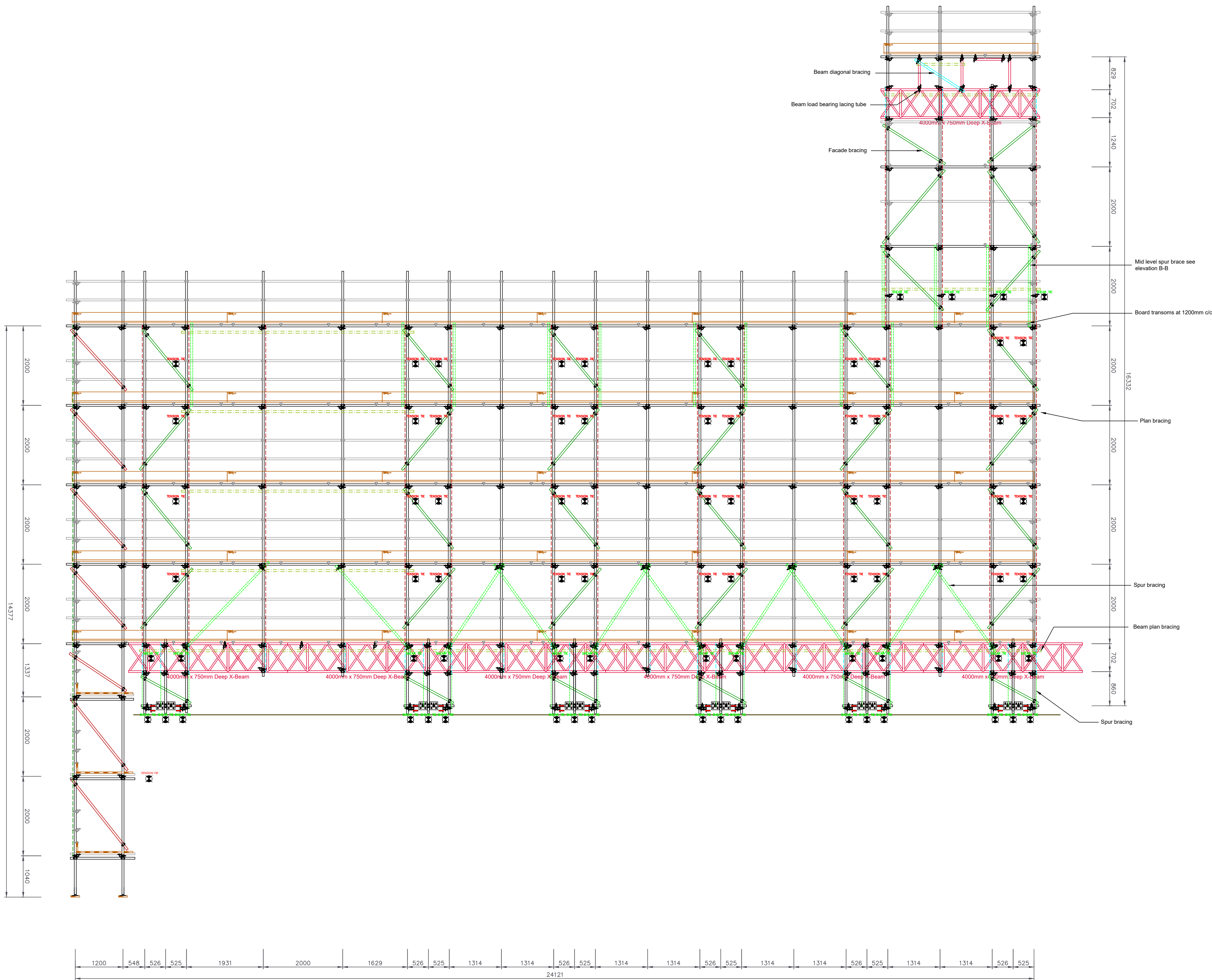
ELEVATION F - F scale 1:50
