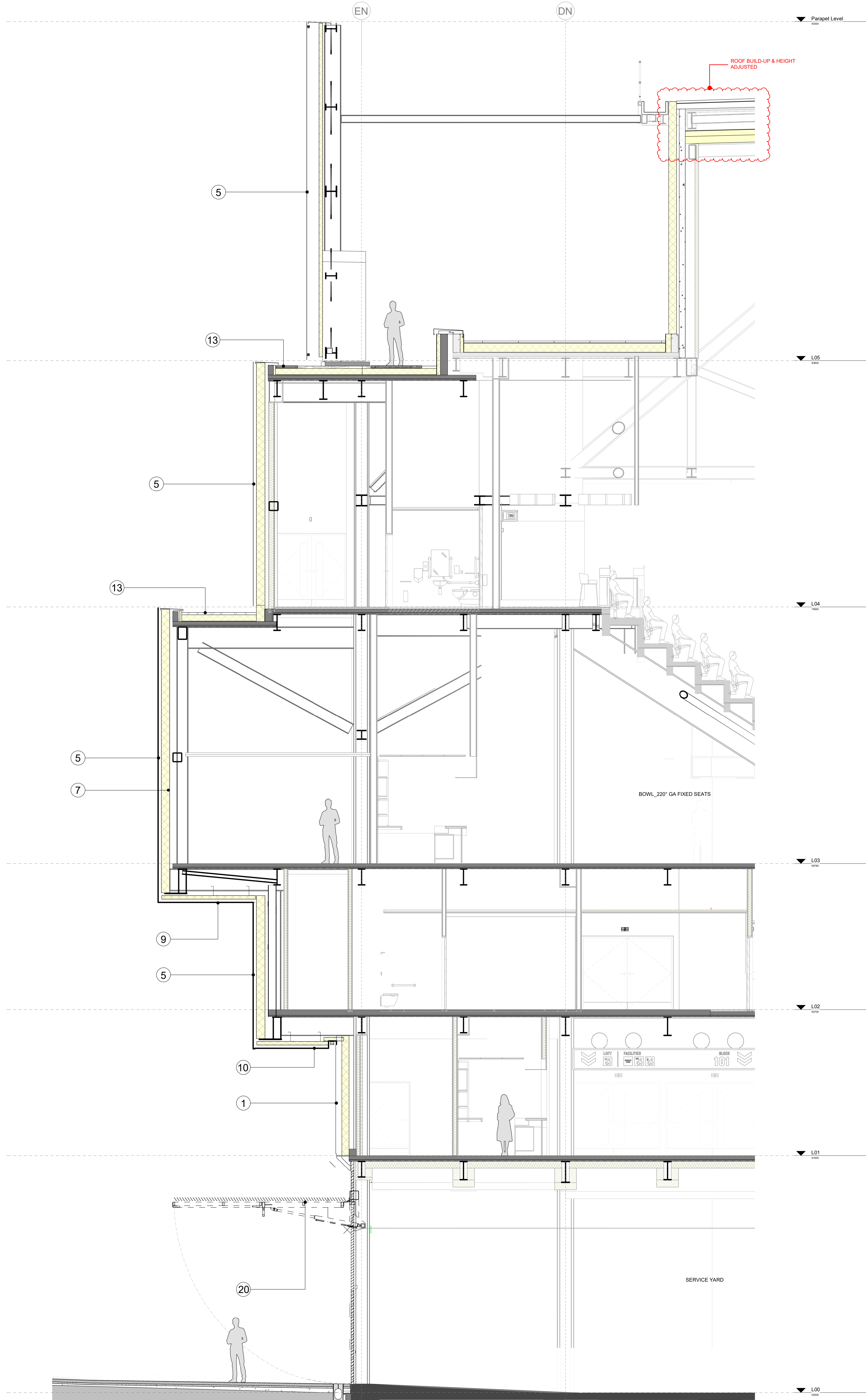
A FACADE SECTION - NORTH 1:50
