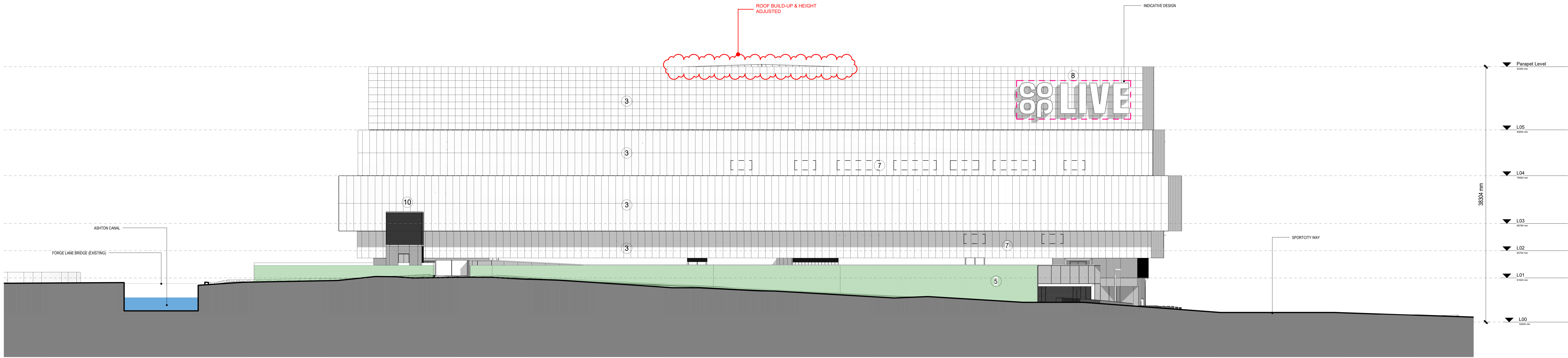
1 ELEVATION - EAST 1:250
