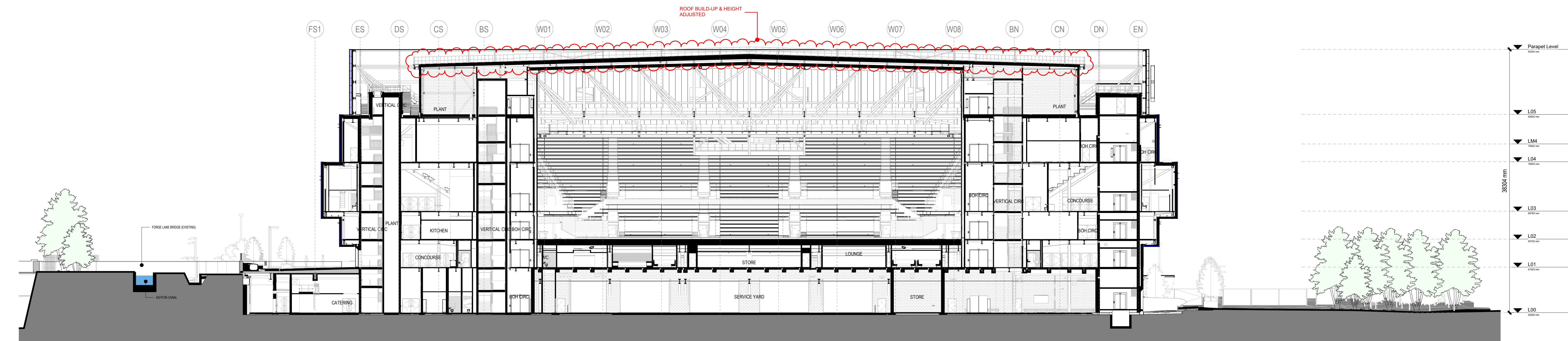
4 PLANNING SECTION - N/S - REAR STAGE TIER 1:250
