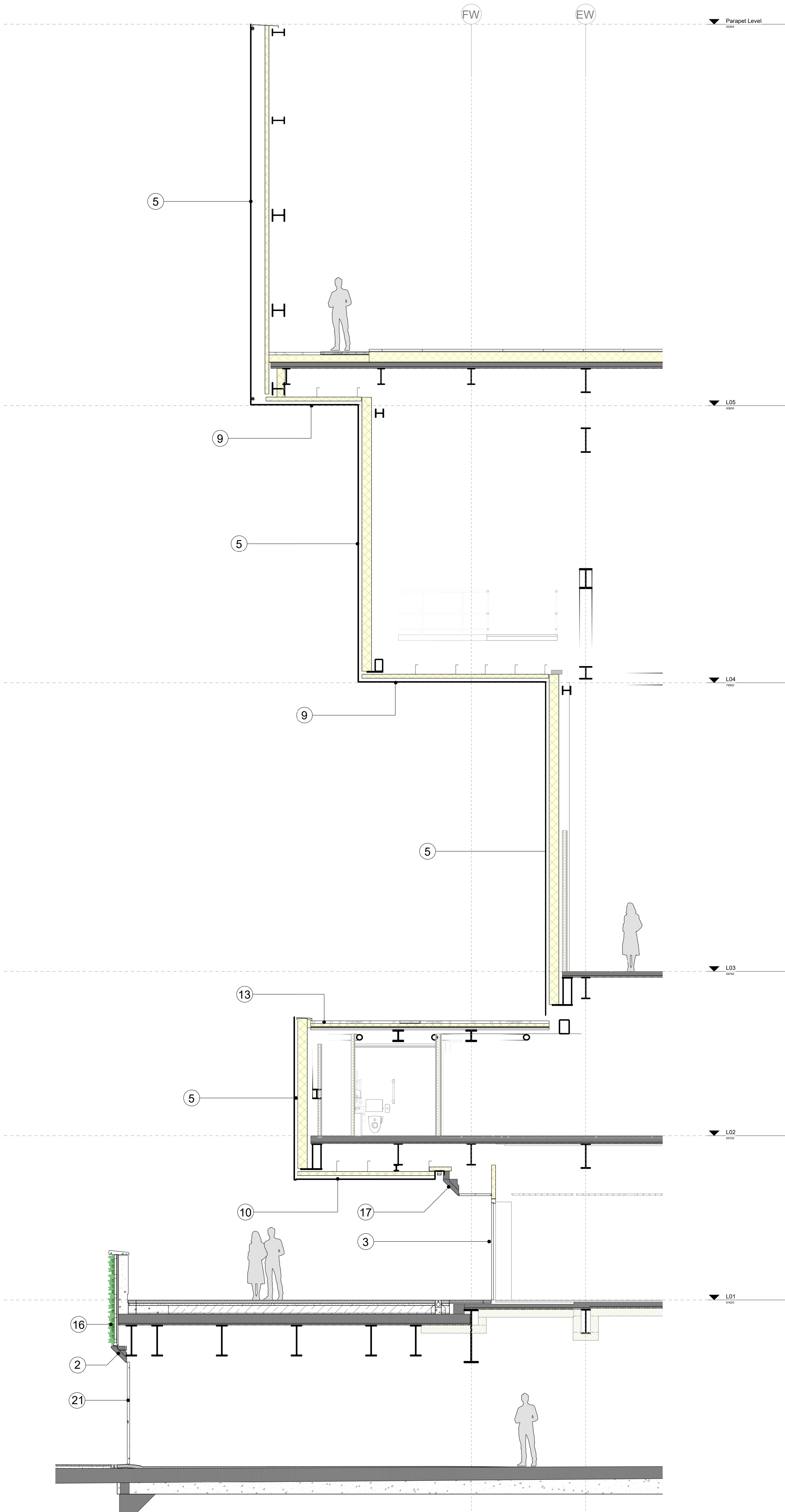
2 FACADE SECTION - WEST 1:50
