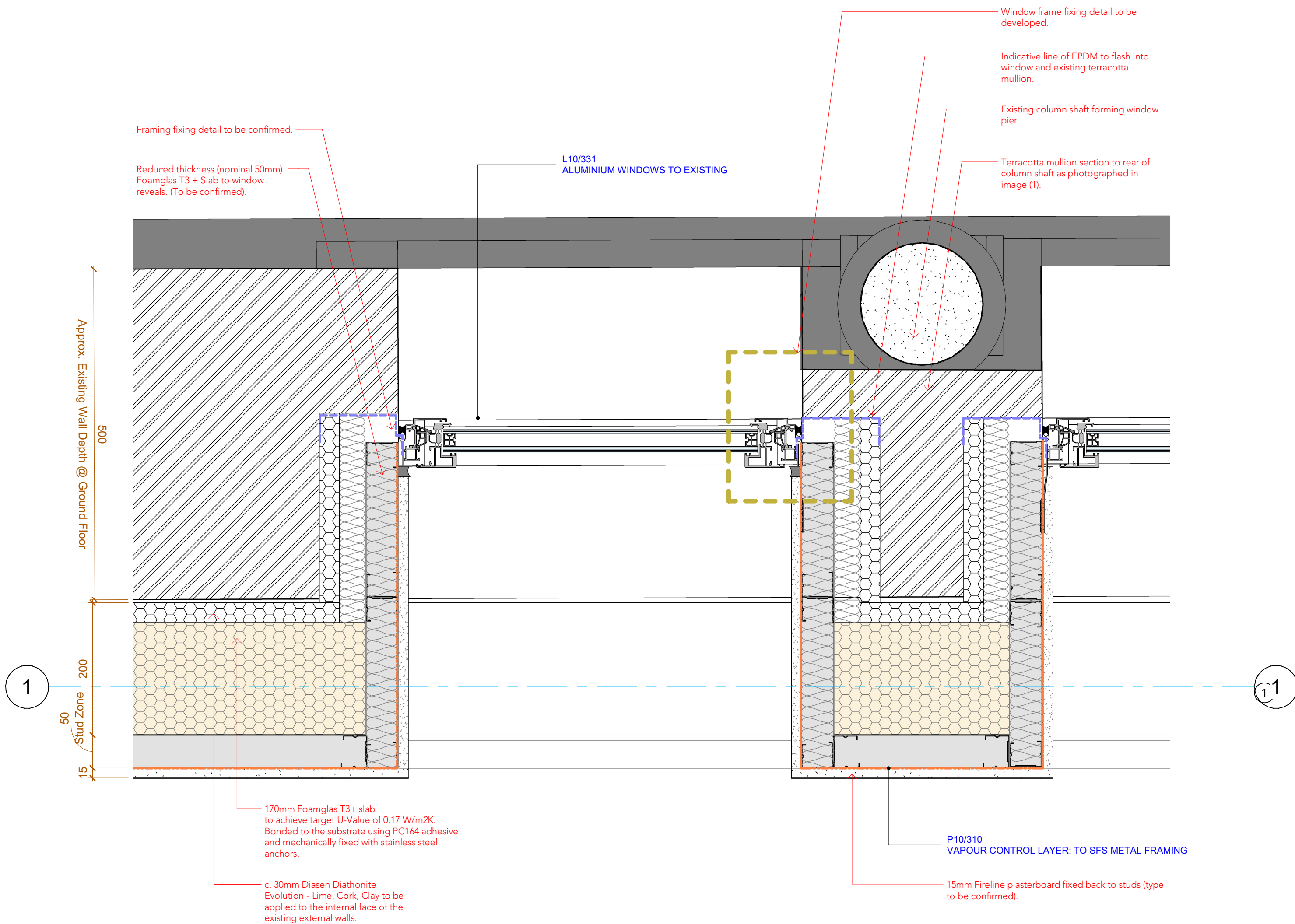
Existing Window Junction with Decorative Pier 1 : 5
