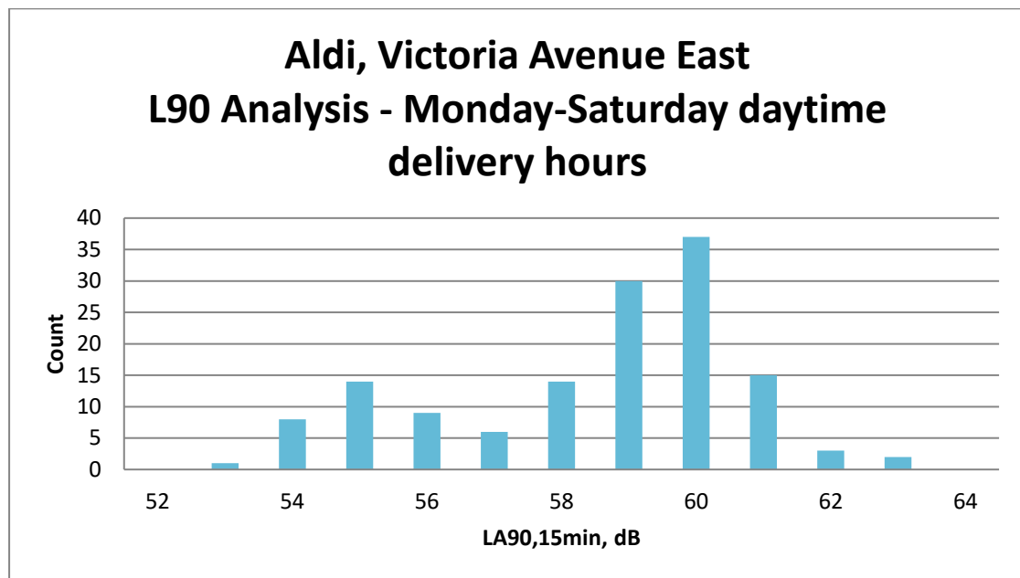
Figure 1 Histogram of L_{A90} background sound pressure levels, Monday-Saturday, 07.00-23.00hrs
