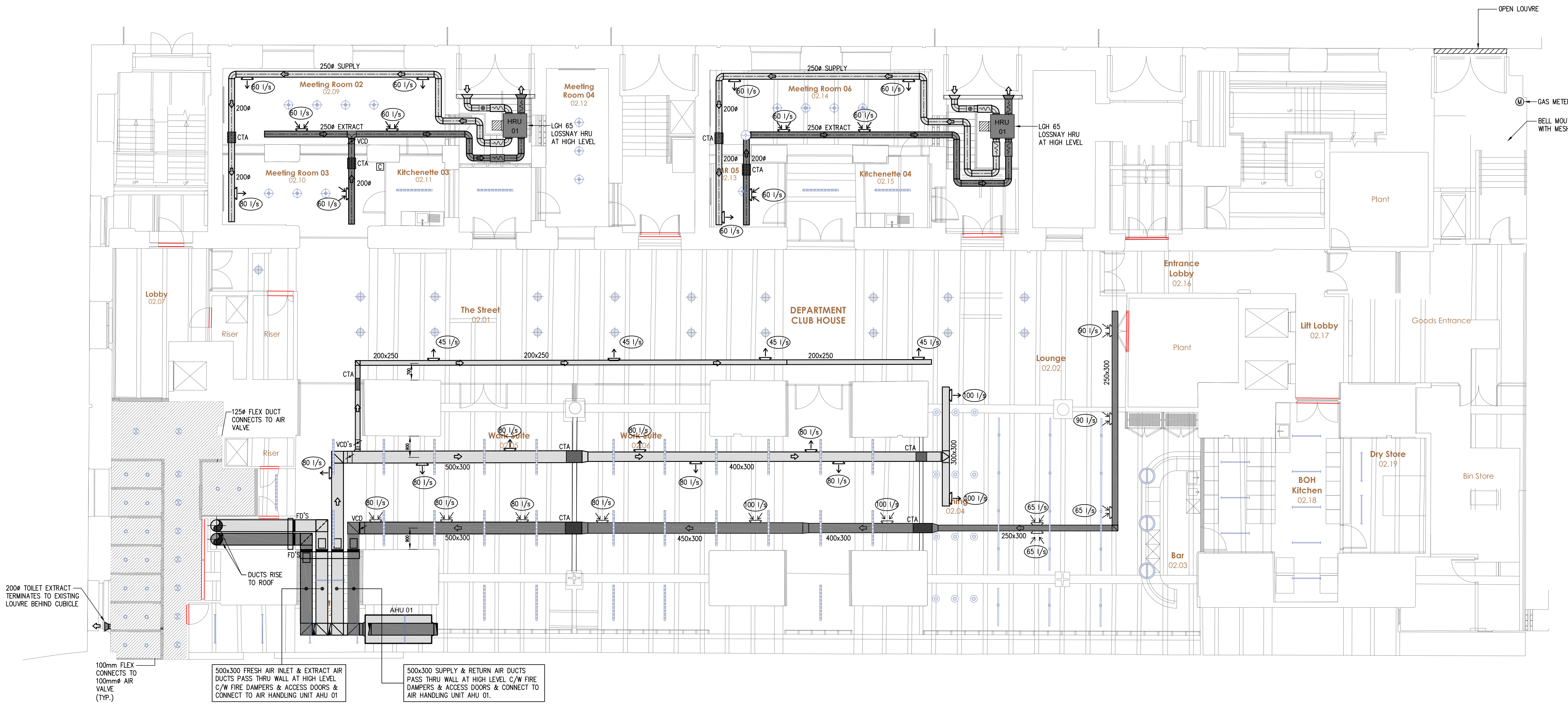
L2 - PRIMARY & SECONDARY DUCTWORK & WC EXTRACT
