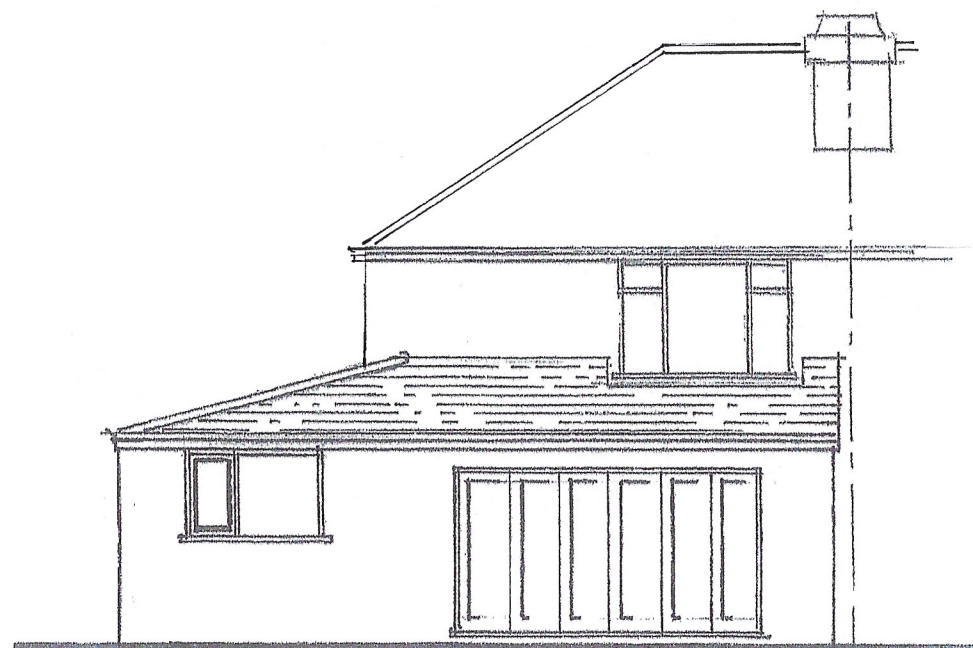
REAR ELEVATION
