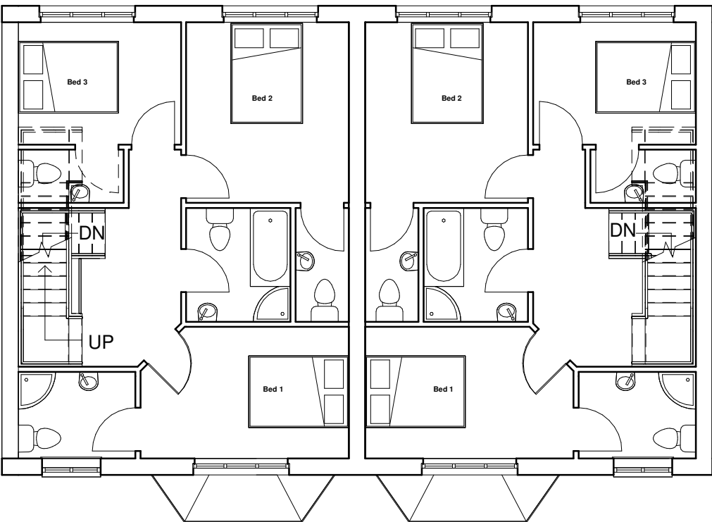
Proposed First Floor 1 : 100
