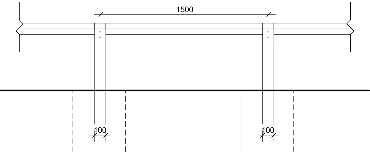
ELEVATION @ 1:20
