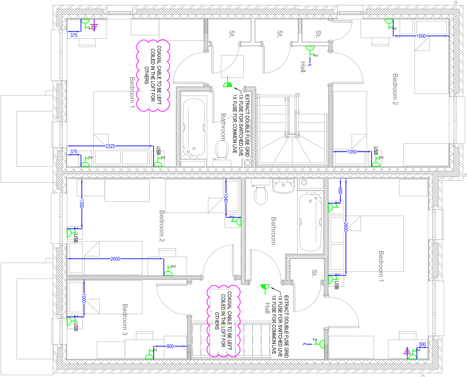
FIRST FLOOR PLOTS 2 & 1
