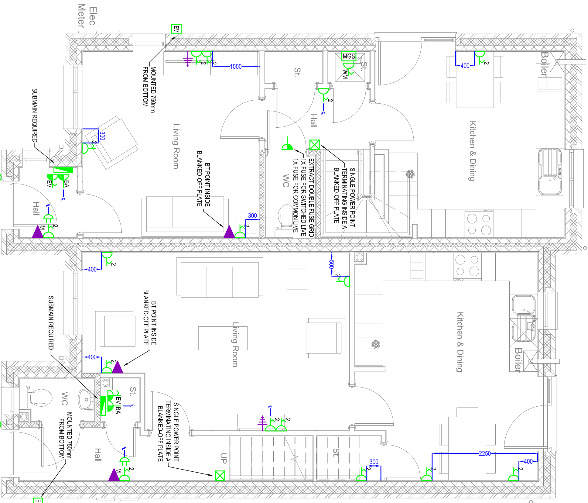
GROUND FLOOR PLOTS 2 & 1
