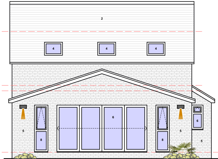
PROPOSED GA REAR ELEVATION @1:100
