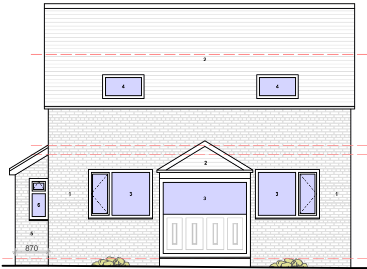
PROPOSED GA FRONT ELEVATION @1:100
