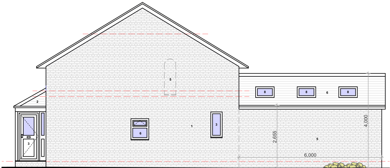
PROPOSED GA SIDE ELEVATION 1 @1:100
