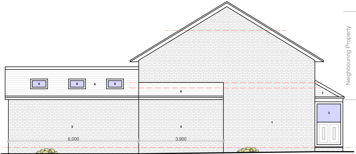
PROPOSED GA SIDE ELEVATION 2 @1:100
