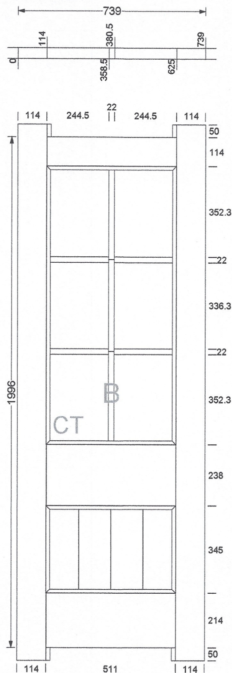
REAR DOORS Door Right Hung
