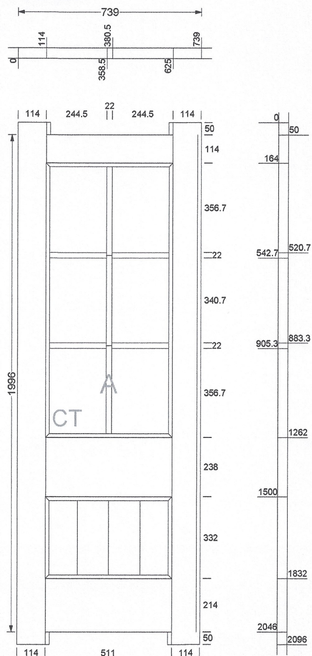
REAR DOORS Door Left Hung
