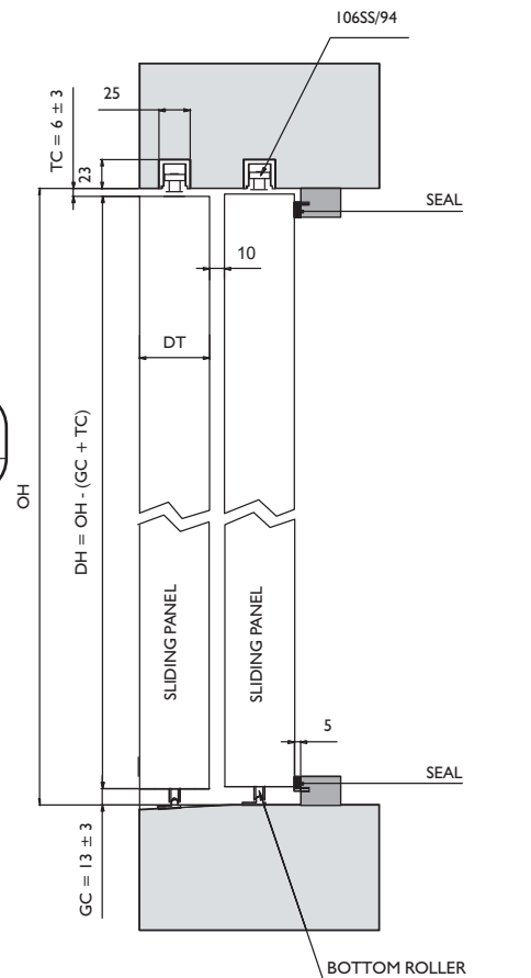
Sliding Panels to One Side
