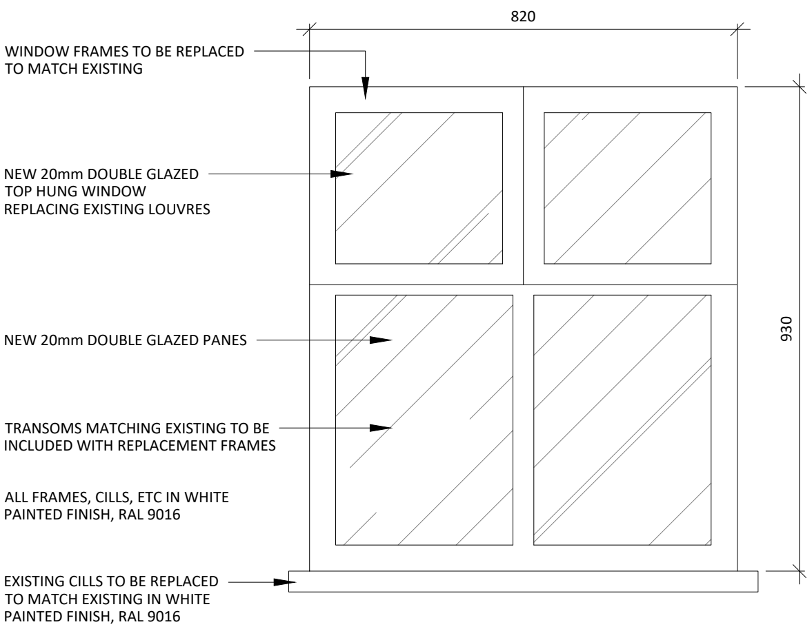
04 4th FLOOR WINDOW W.5.14 - TYPE I 518 SCALE 1:10 PROPOSED ELEVATION
