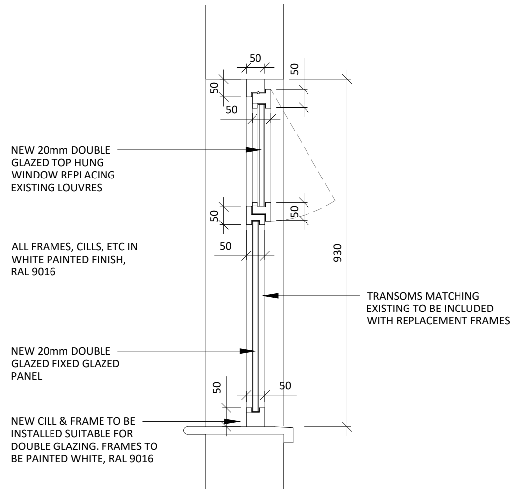
05 4th FLOOR WINDOW W.5.14 - TYPE I 518 SCALE 1:10 PROPOSED SECTION
