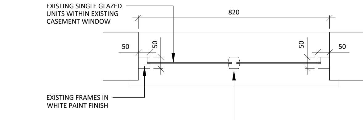
03 4th FLOOR WINDOW W.5.14 - TYPE I 518 SCALE 1:10 EXISTING PLAN SECTION
