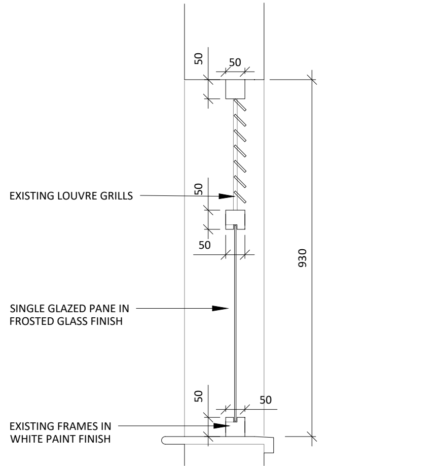
02 4th FLOOR WINDOW W.5.14 - TYPE I 518 SCALE 1:10 EXISTING SECTION
