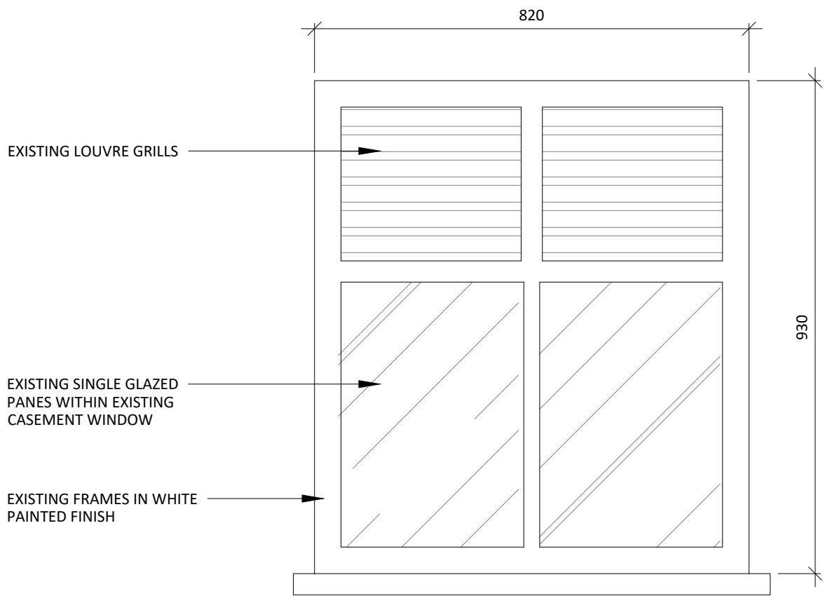
01 4th FLOOR WINDOW W.5.14 - TYPE I 518 SCALE 1:10 EXISTING ELEVATION
