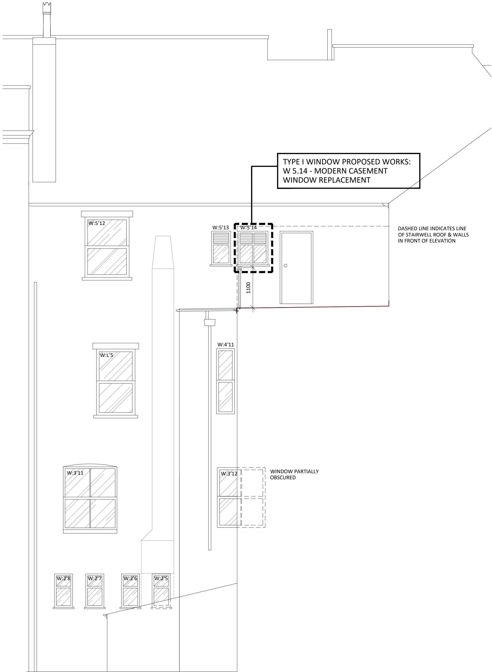
09 COURTYARD ELEVATION 518 SCALE 1:50
