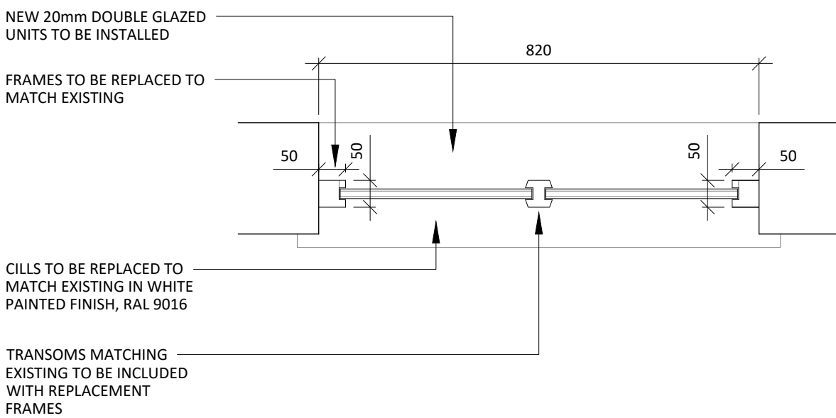
06 4th FLOOR WINDOW W.5.14 - TYPE I 518 SCALE 1:10 PROPOSED PLAN SECTION
