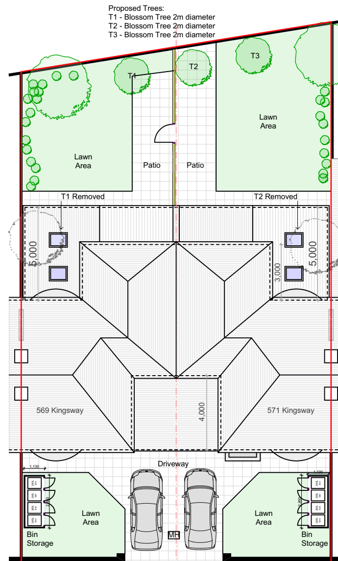
PROPOSED GA SITE PLAN @1:200
