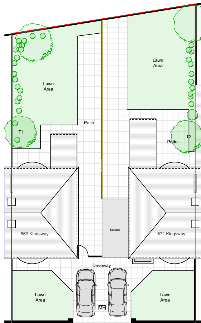
EXISTING GA SITE PLAN @1:200
