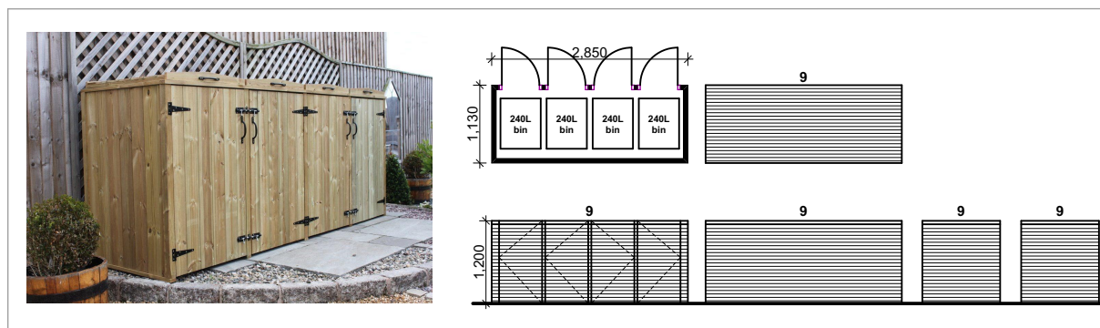
PROPOSED GA ELEVATIONS & FLOOR PLANS OF WASTE BINS STORAGE @ 1:100
