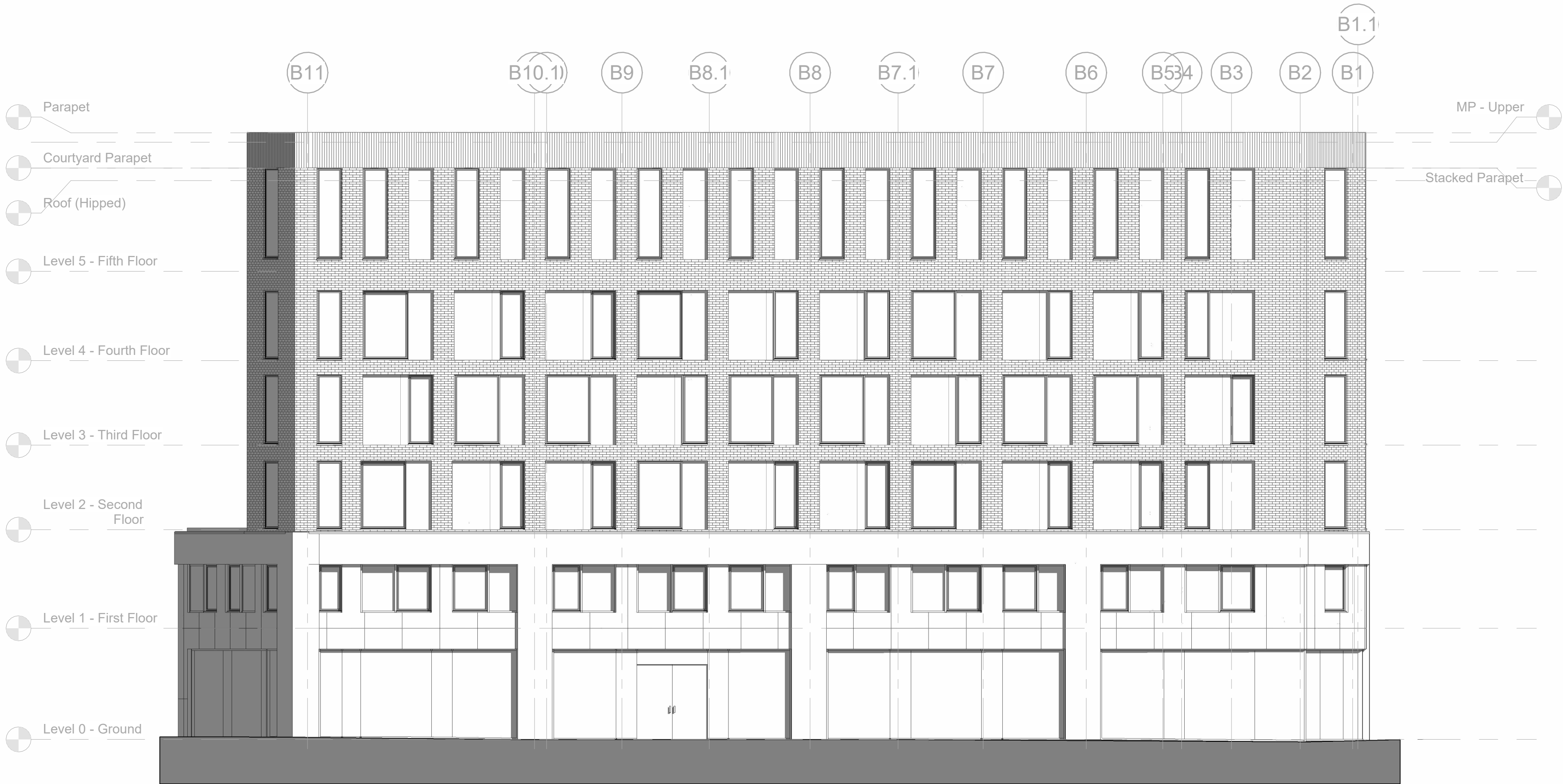
Existing Stockport Road Elevation 1 : 100
