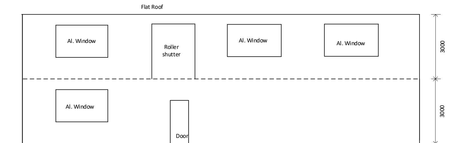
EXISTING SIDE ELEVATION from Shop No. 37
