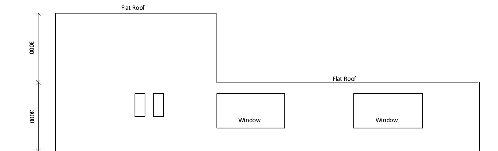
EXISTING SIDE ELEVATION From 39D No change will Occur
