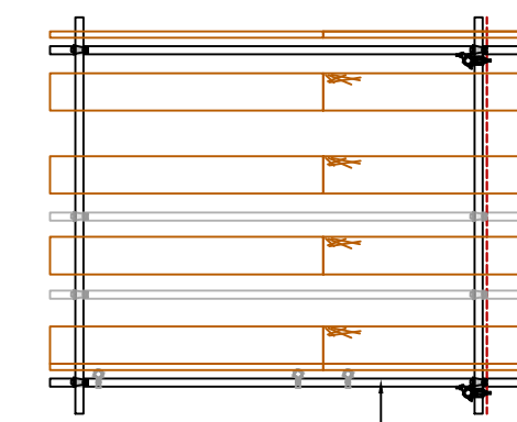
TYPICAL RANCH BOARDING DETAIL scale 1:50
