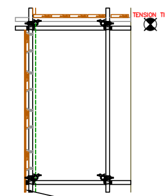
TYPICAL RANCH BOARDING DETAIL scale 1:50
