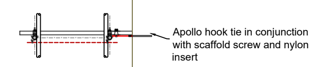
TYPICAL RANCH BOARDING DETAIL scale 1:50
