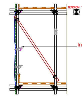
TYPICAL CLADDING DETAIL scale 1:50
