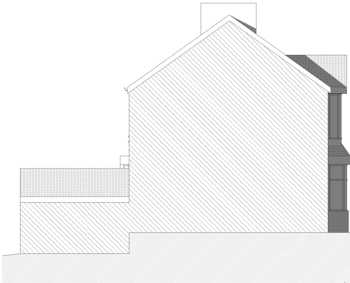
6 Existing West Elevation
