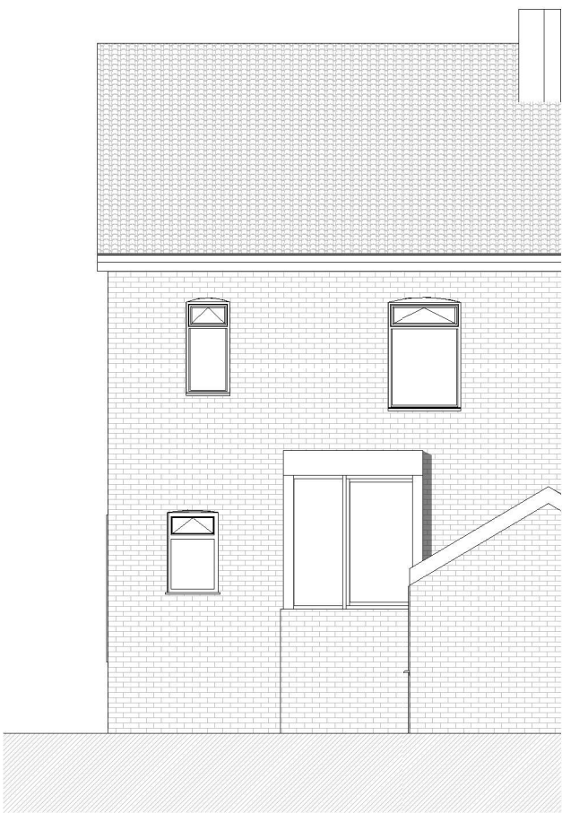
4 Existing North Elevation
