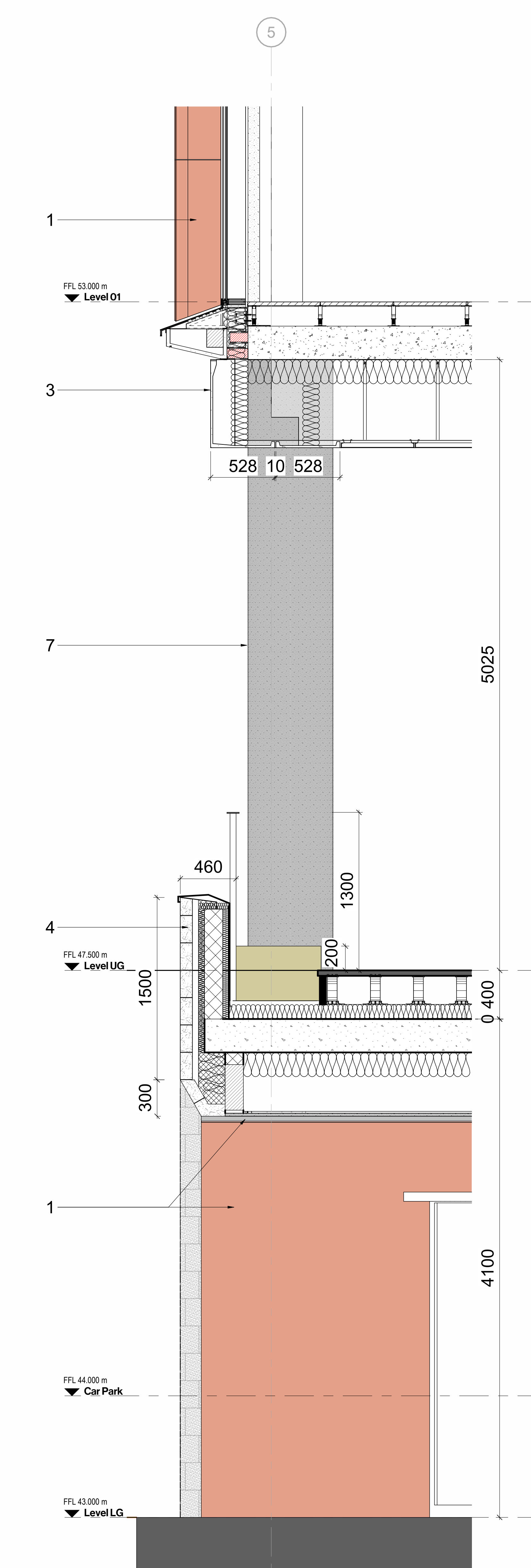
2 Lower Ground Bay Study - Section
