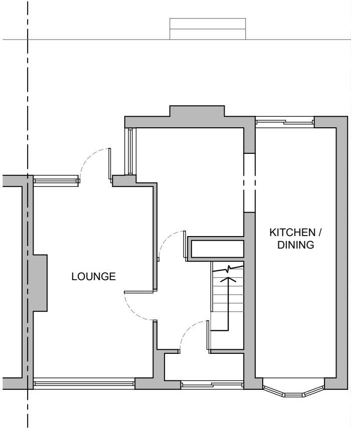
GROUND FLOOR 1:100
