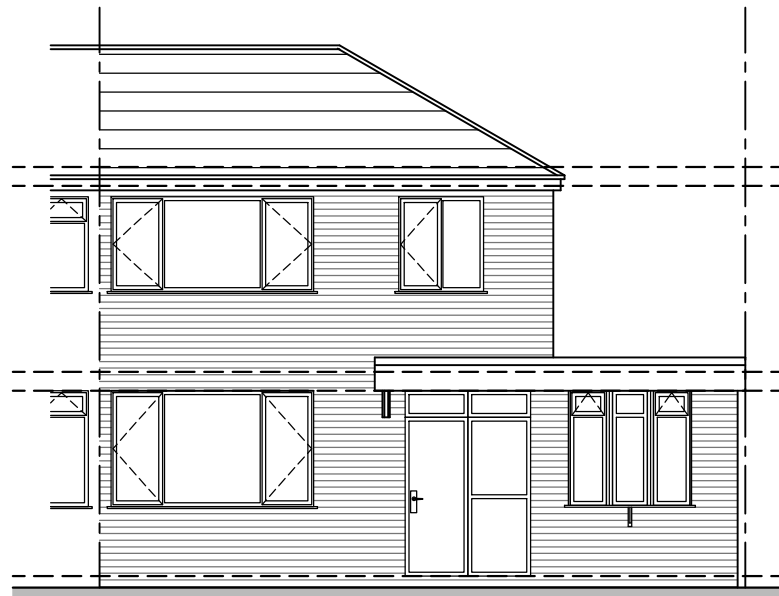
FRONT ELEVATION 1:100
