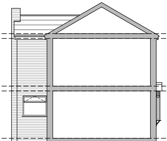
SIDE ELEVATION 1:100
