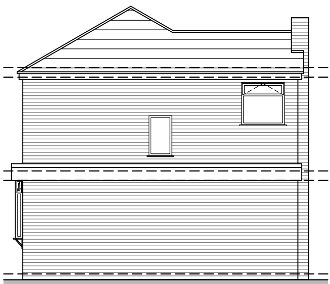
SIDE ELEVATION 1:100
