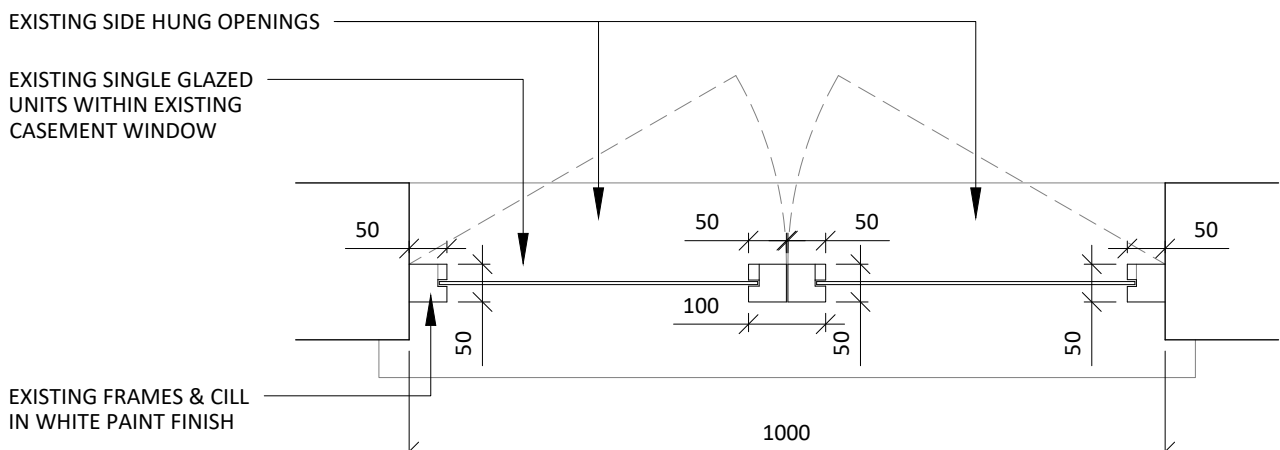
06 4th FLOOR WINDOW W.L.2 - TYPE K 520 SCALE 1:10 PROPOSED PLAN SECTION
