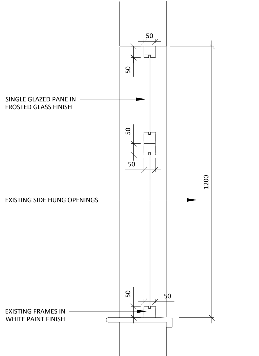
02 4th FLOOR WINDOW W.L.2 - TYPE K 520 SCALE 1:10 EXISTING SECTION
