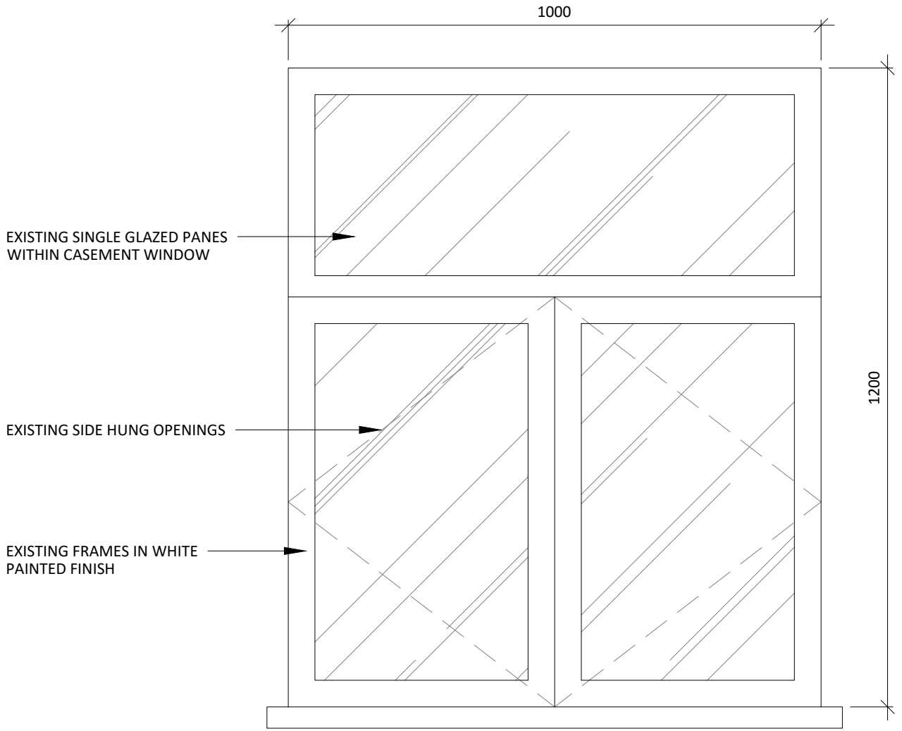
01 4th FLOOR WINDOW W.L.2 - TYPE K 520 SCALE 1:10 EXISTING ELEVATION
