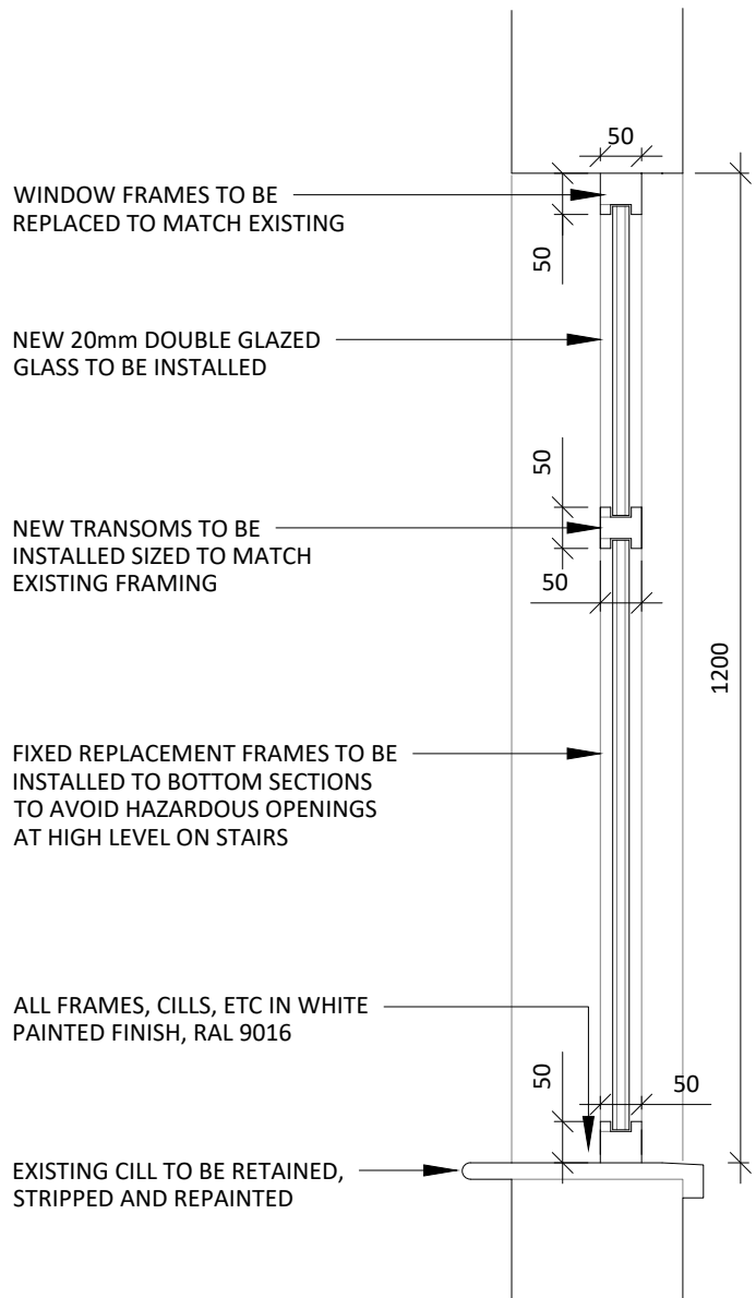
05 4th FLOOR WINDOW W.L.2 - TYPE K 520 SCALE 1:10 PROPOSED SECTION
