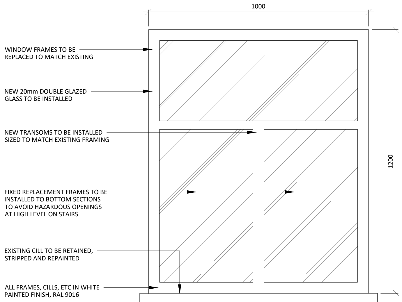
04 4th FLOOR WINDOW W.L.2 - TYPE K 520 SCALE 1:10 PROPOSED ELEVATION
