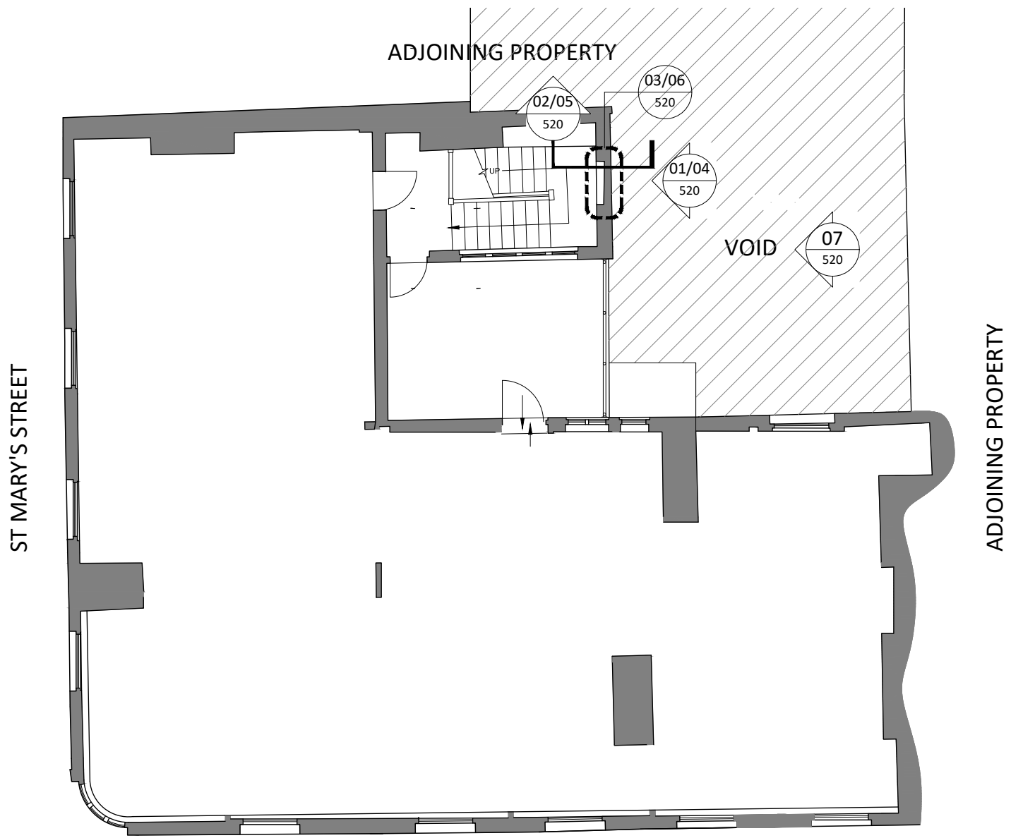
10 THIRD FLOOR REFERENCE PLAN 520 SCALE 1:100
