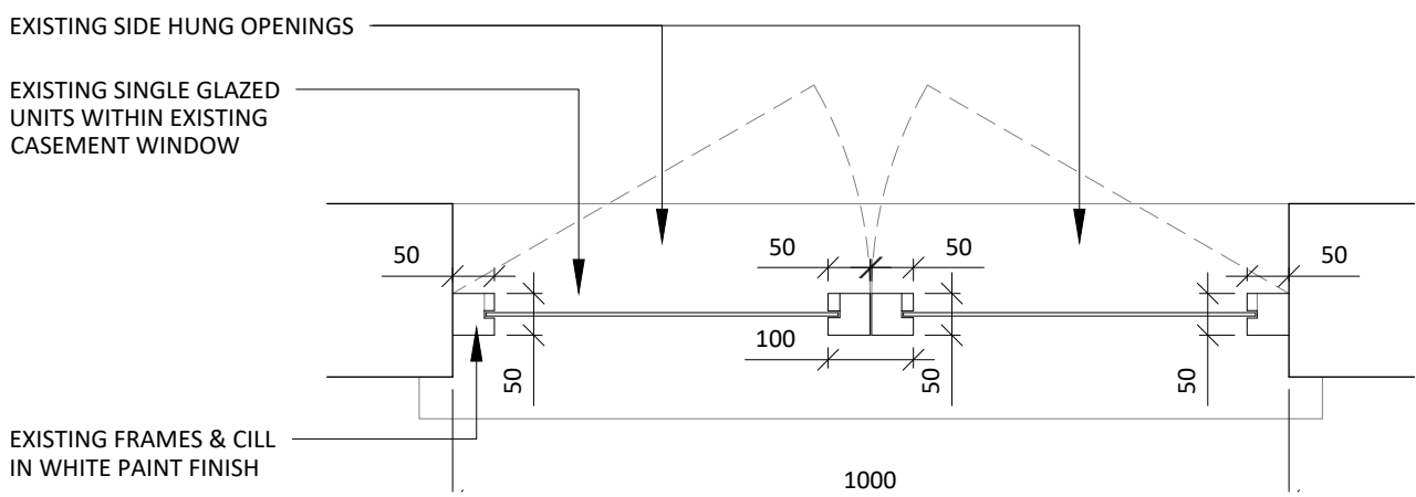
03 4th FLOOR WINDOW W.L.2 - TYPE K 520 SCALE 1:10 EXISTING PLAN SECTION
