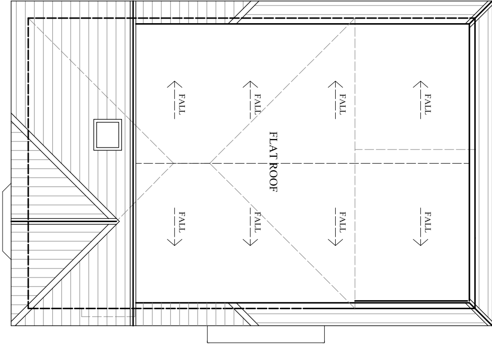
PROPOSED ROOF PLAN 1:100@A4
