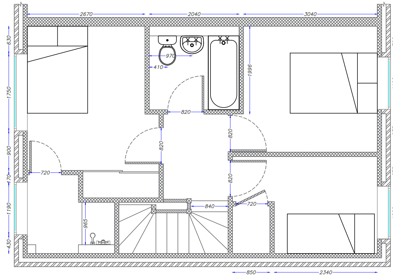
Existing 1st Floor Layout
