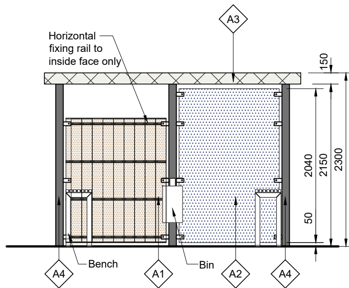
FRONT ELEVATION
