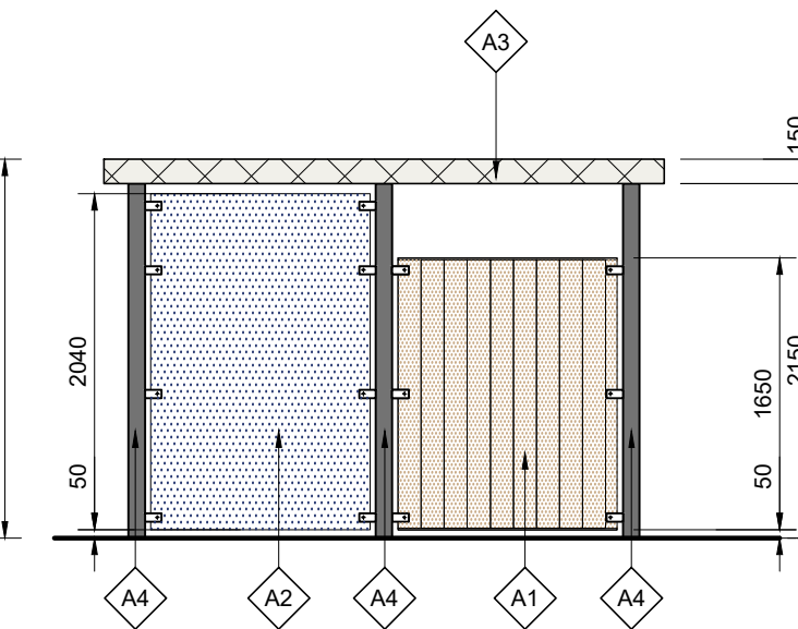
REAR ELEVATION
