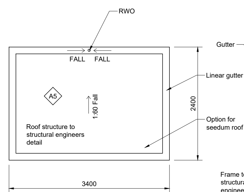
ROOF PLAN
