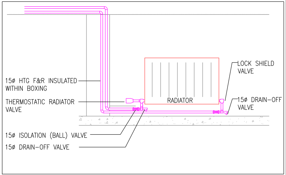
GENERAL ARRANGEMENT OF VALVES AND PIPEWORK CONNECTIONS TO RADIATORS
