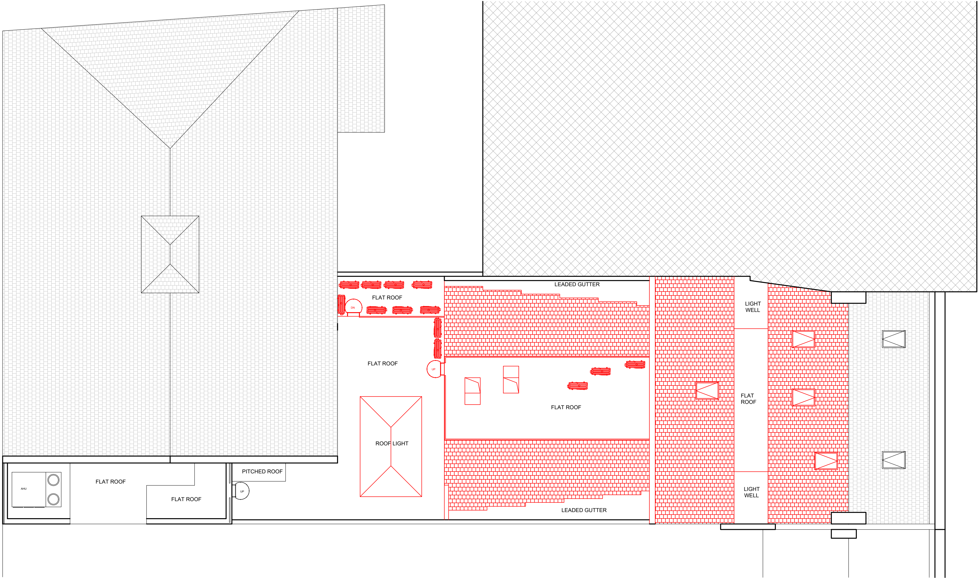
ROOF DEMOLITION PLAN SCALE 1:100
