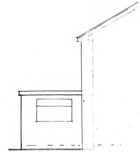
SIDE ELEVATION (EXISTING)
