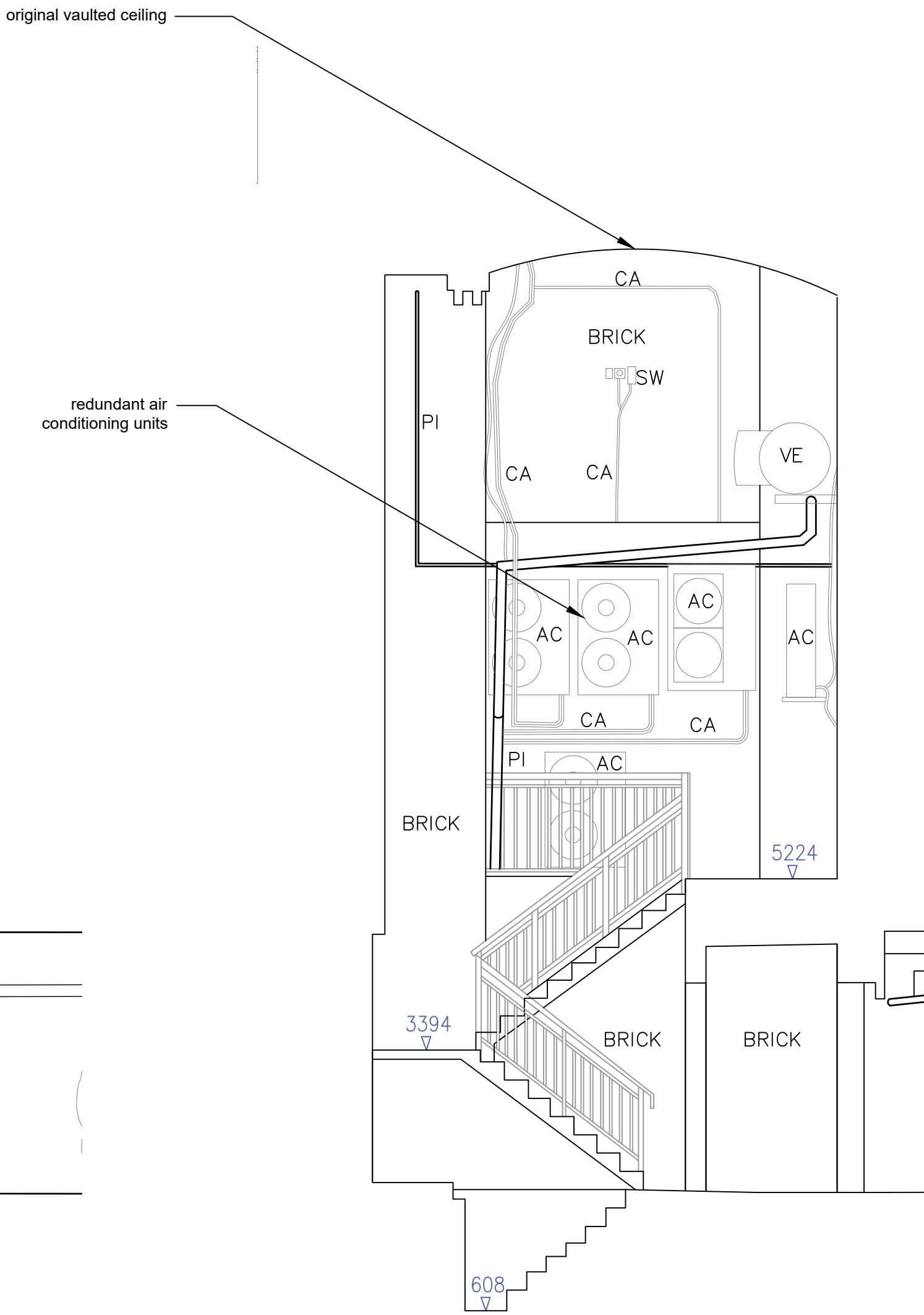
B Existing Section
